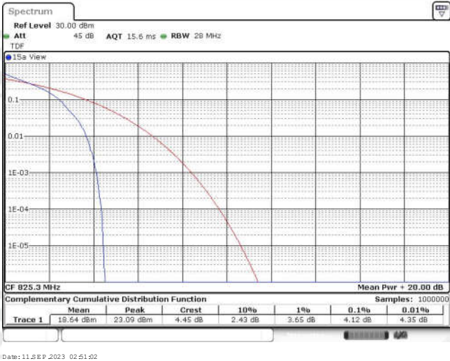
Band26-5MHz-QPSK-26803-25RB#0
