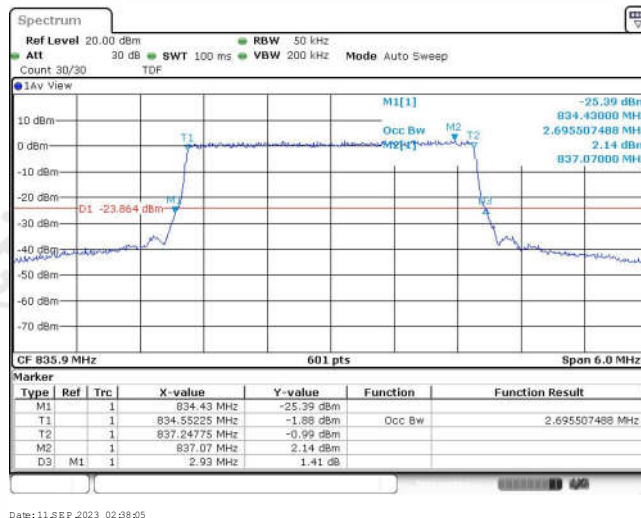
Band26-3MHz-16QAM-27025-15RB#0-2.696
