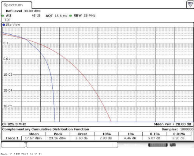
Band26-5MHz-16QAM-26803-25RB#0
