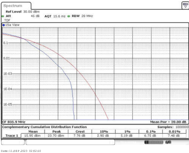
Band26-5MHz-16QAM-26909-25RB#0
