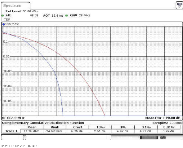
Band26-3MHz-QPSK-26909-15RB#0
