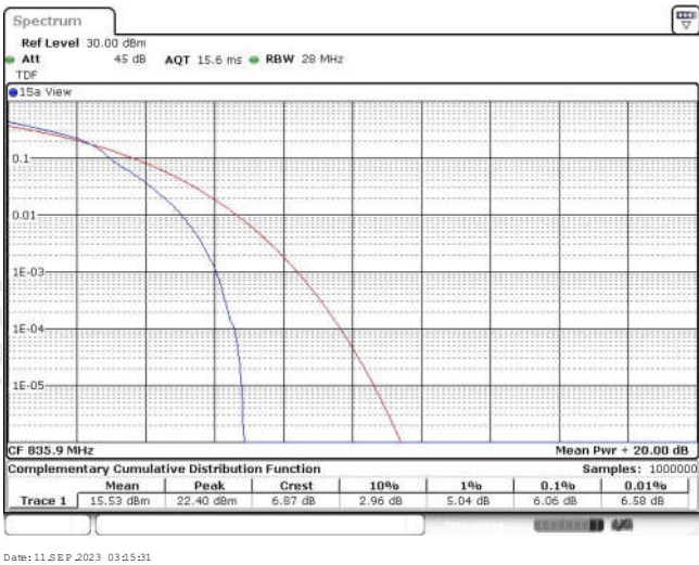
Band26-15MHz-16QAM-26909-75RB#0
