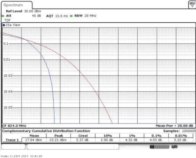
Band26-3MHz-16QAM-26793-15RB#0
