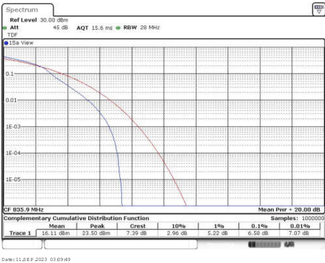
Band26-10MHz-16QAM-26909-50RB#0
