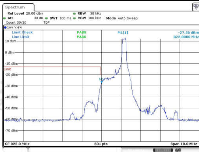
Band26-1.4MHz-16QAM-26785-6RB#0
