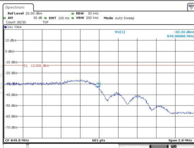
Band26-3MHz-16QAM-27025-1RB#0
