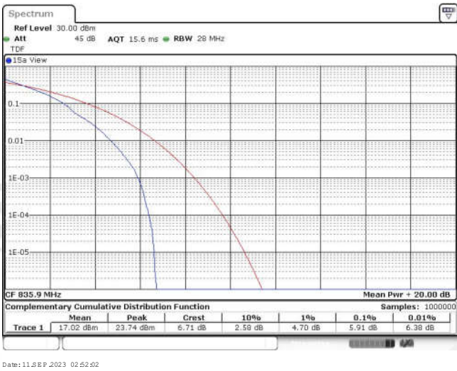
Band26-5MHz-QPSK-26909-25RB#0
