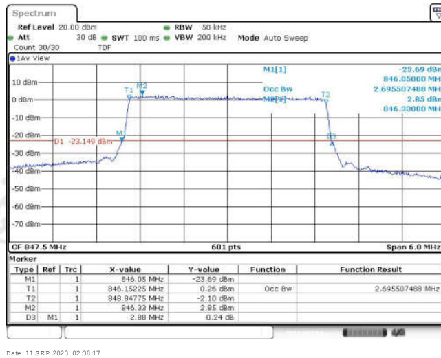
Band26-3MHz-16QAM-26793-15RB#0-2.696
