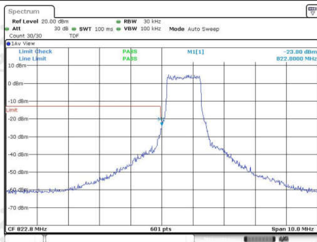
Band26-1.4MHz-16QAM-26785-6RB#0
