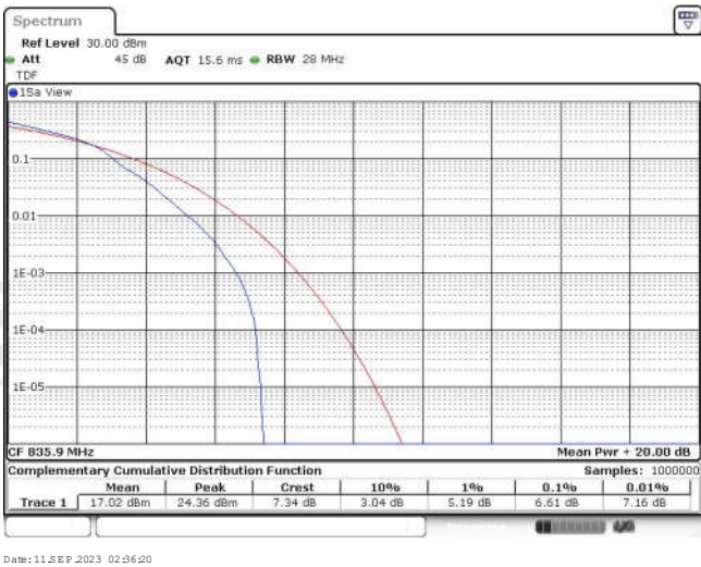
Band26-1.4MHz-16QAM-26909-6RB#0
