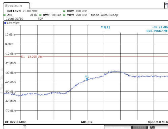
Band26-5MHz-QPSK-26803-25RB#0
