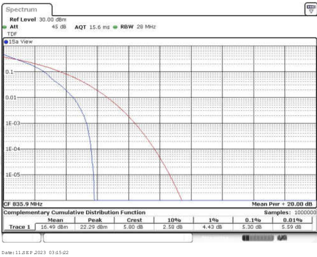
Band26-15MHz-QPSK-26909-75RB#0
