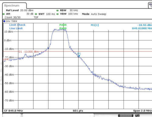
Band26-1.4MHz-QPSK-27033-6RB#0
