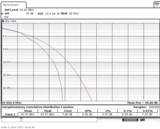
Band26-3MHz-16QAM-26909-15RB#0
