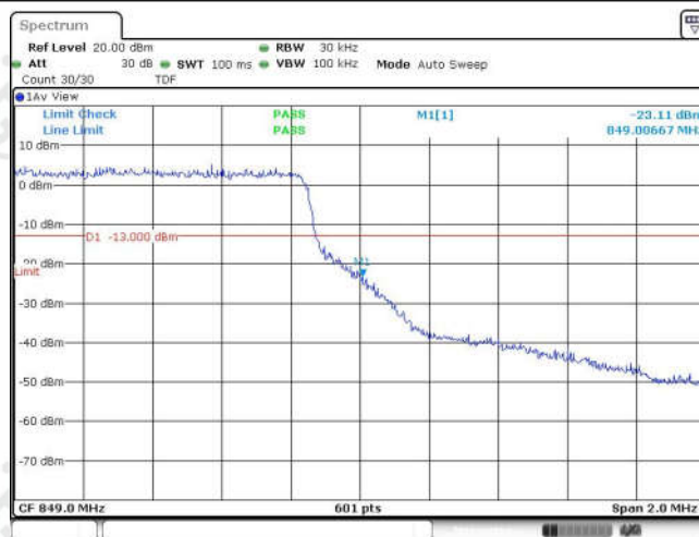
Band26-1.4MHz-16QAM-27033-6RB#0
