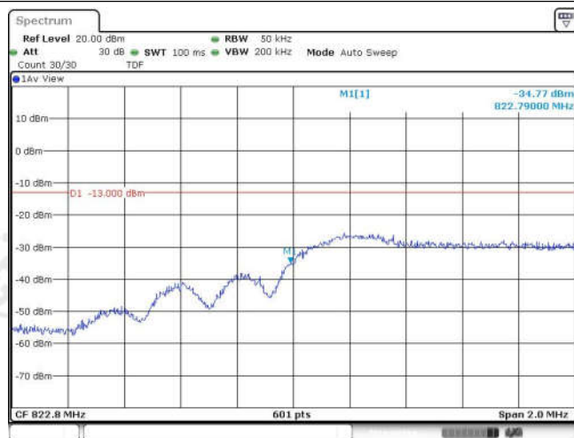
Band26-3MHz-16QAM-26793-15RB#0
