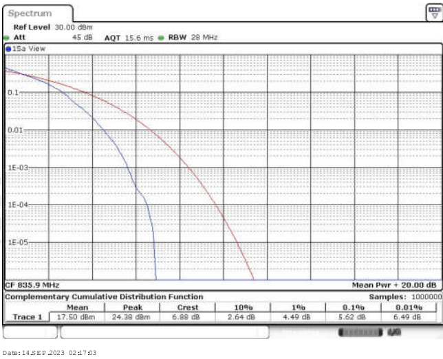
Band26-1.4MHz-QPSK-26909-6RB#0
