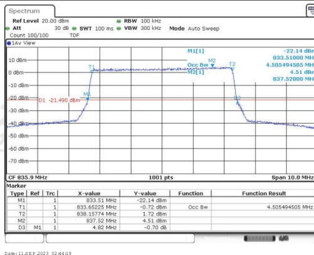
Band26-5MHz-QPSK-27015-25RB#0-4.505
