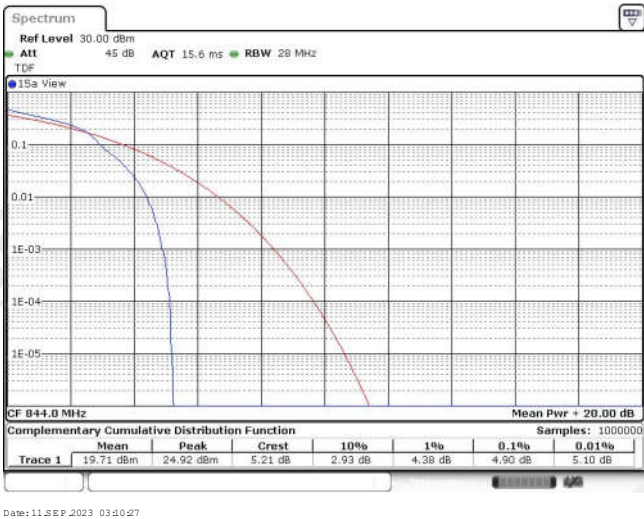
Band26-10MHz-16QAM-26990-50RB#0
