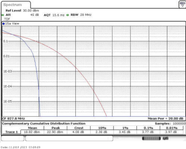
Band26-10MHz-QPSK-26828-50RB#0
