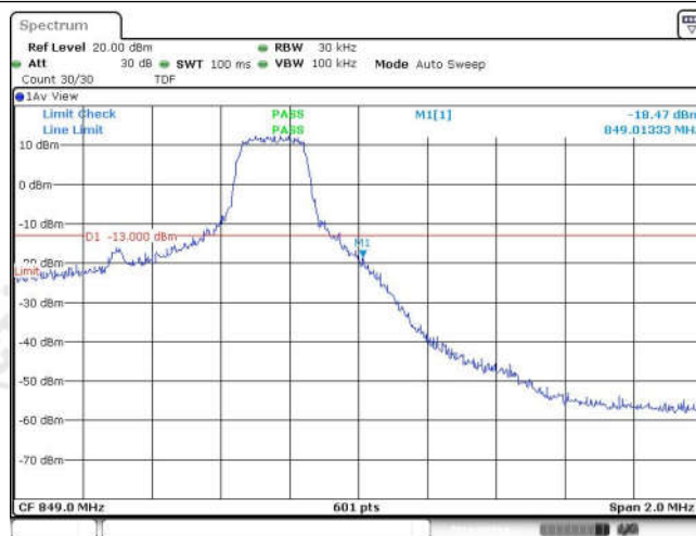
Band26-1.4MHz-16QAM-27033-6RB#0
