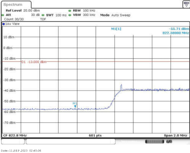
Band26-5MHz-QPSK-26803-1RB#24
