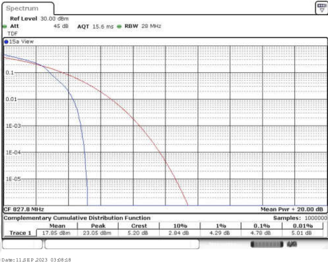
Band26-10MHz-16QAM-26828-50RB#0
