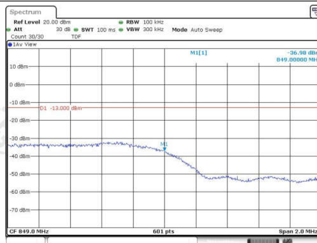
Band26-5MHz-QPSK-27015-1RB#0
