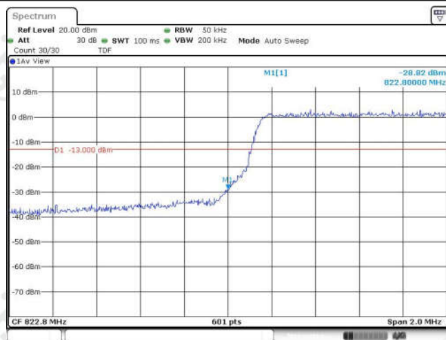
Band26-3MHz-16QAM-26793-15RB#0
