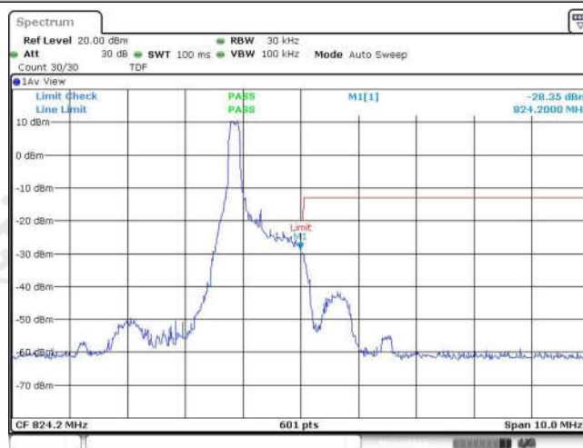
Band26-1.4MHz-16QAM-26785-1RB#0
