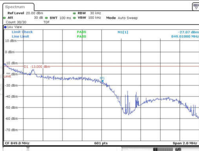
Band26-1.4MHz-16QAM-27033-1RB#0
