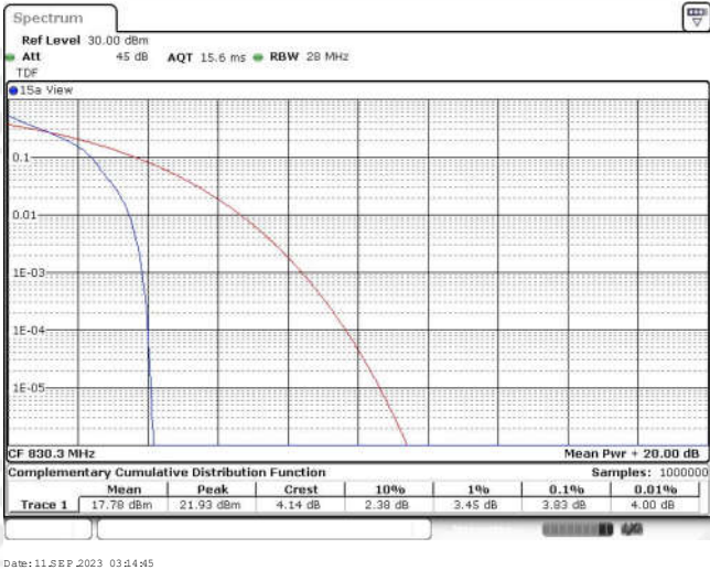
Band26-15MHz-QPSK-26853-75RB#0
