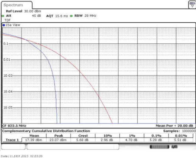
Band26-1.4MHz-16QAM-26785-6RB#0
