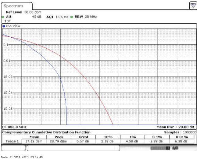
Band26-10MHz-QPSK-26909-50RB#0
