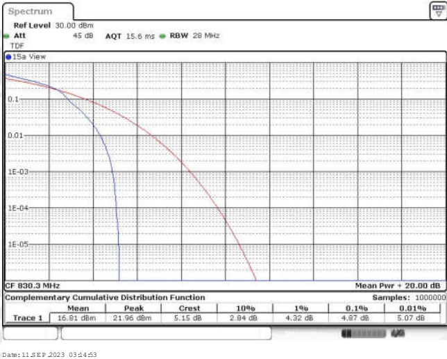
Band26-15MHz-16QAM-26853-75RB#0
