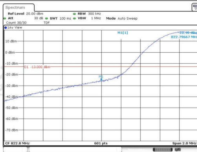
Band26-15MHz-QPSK-26853-1RB#0
