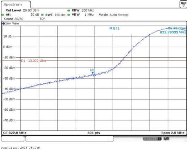
Band26-15MHz-16QAM-26853-1RB#74
