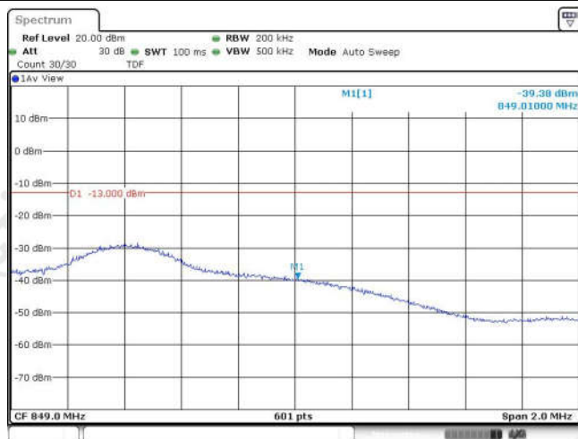
Band26-10MHz-16QAM-26990-1RB#0
