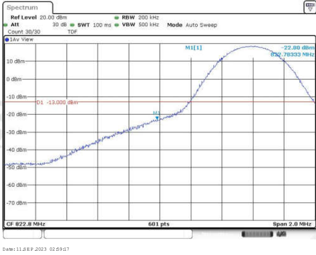
Band26-10MHz-QPSK-26828-1RB#49
