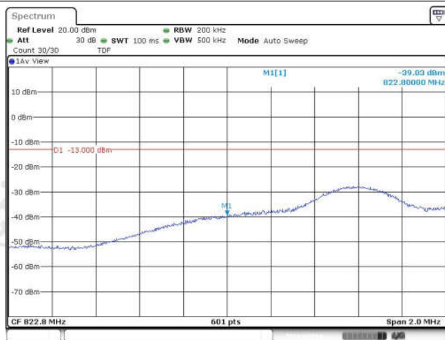
Band26-10MHz-16QAM-26828-50RB#0
