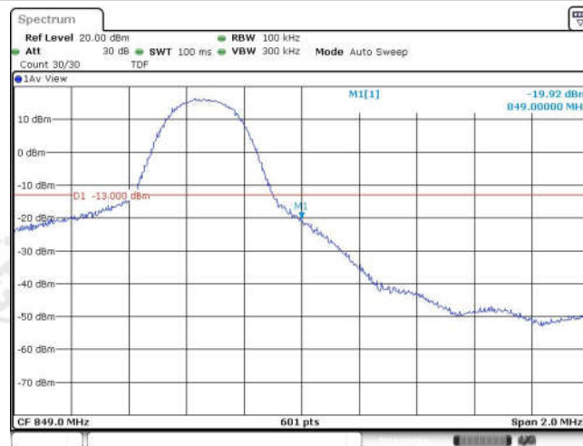
Band26-5MHz-QPSK-27015-25RB#0
