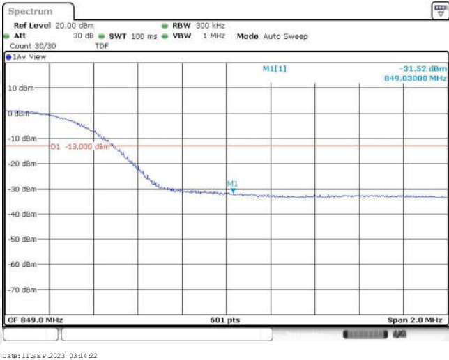
Band26-15MHz-16QAM-26853-1RB#0
