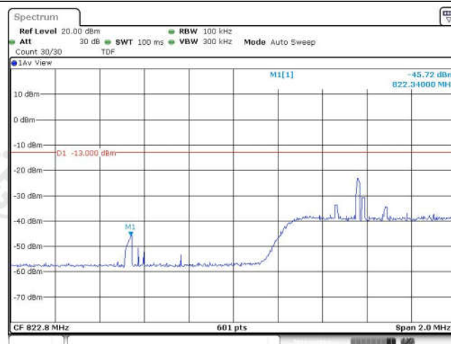
Band26-5MHz-16QAM-26803-1RB#0
