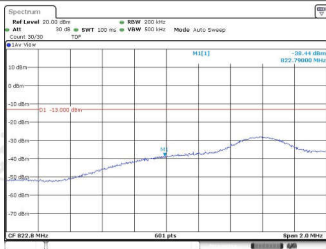
Band26-10MHz-QPSK-26828-50RB#0
