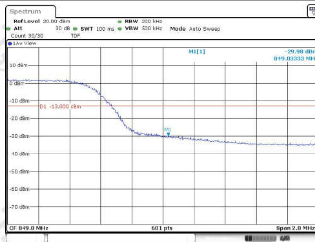
Band26-10MHz-QPSK-26990-50RB#0
