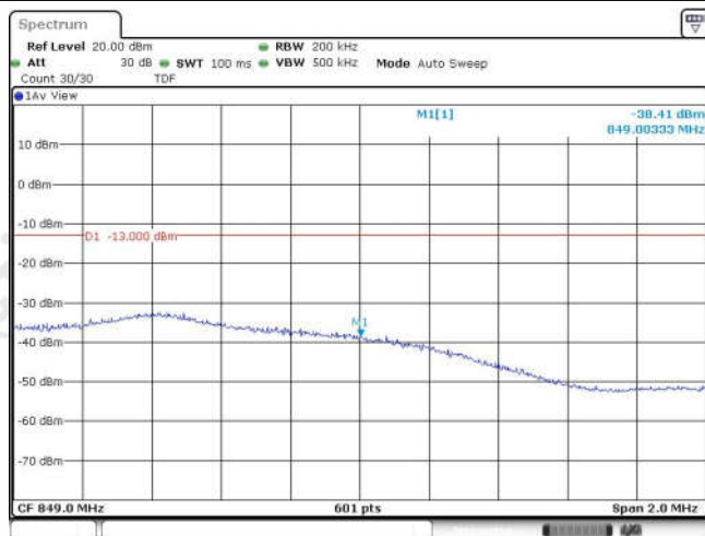
Band26-10MHz-QPSK-26990-1RB#0
