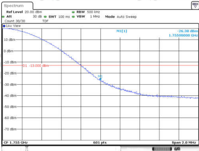
Band4-20MHz-16QAM-20300-1RB#99
