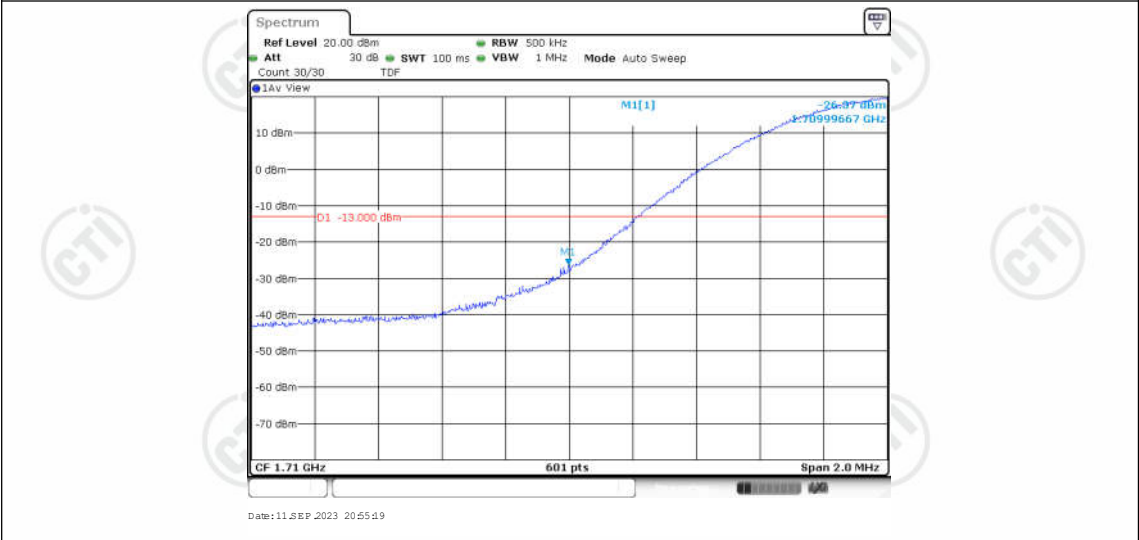
Band4-20MHz-16QAM-20050-1RB#99
