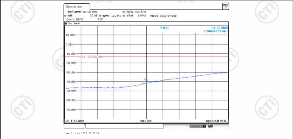
Band4-20MHz-16QAM-20050-100RB#0
