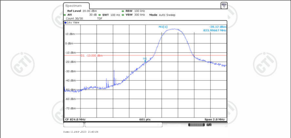
Band5-5MHz-16QAM-20425-1RB#24
