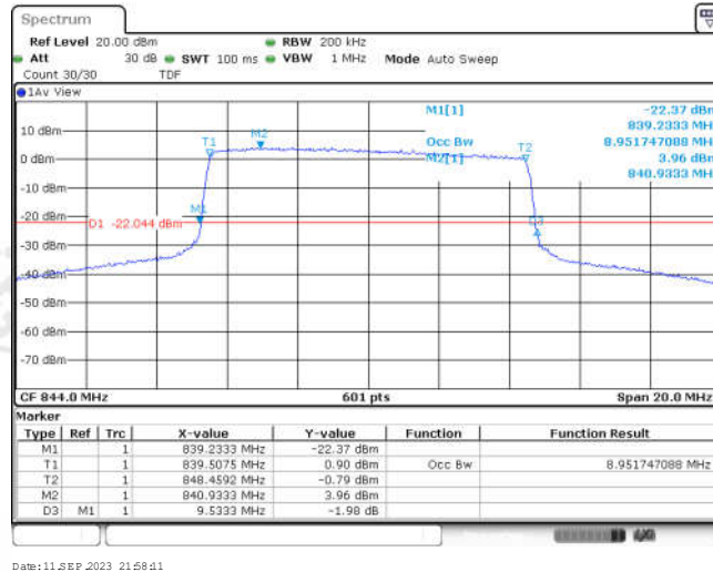
Band5-10MHz-16QAM-20450-50RB#0-8.952
