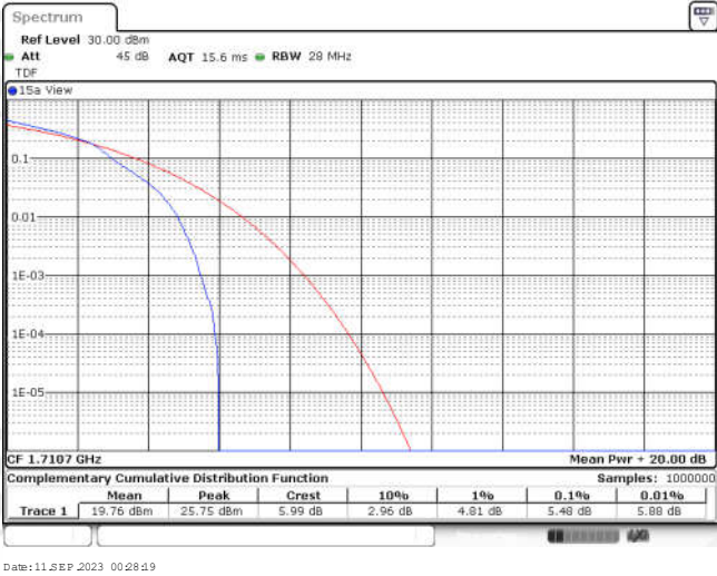
Band66-1.4MHz-16QAM-131979-6RB#0
