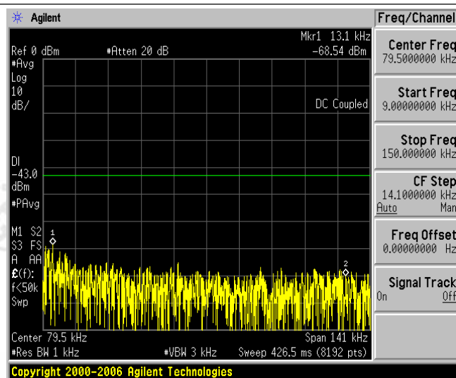
Band2-9262-3-10000~20000MHz
