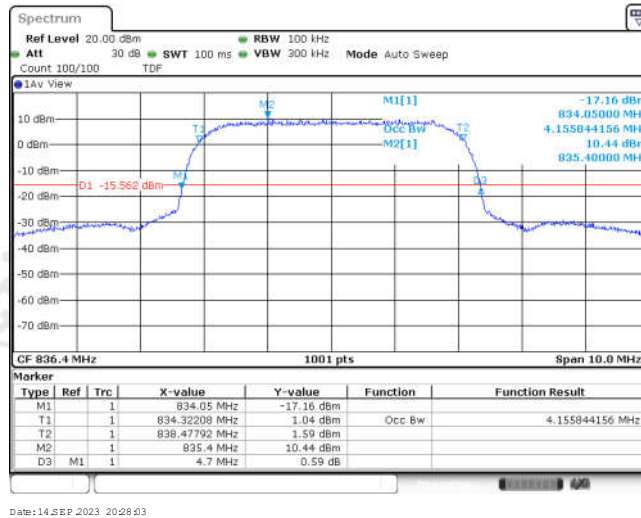
Band5-4182-4
