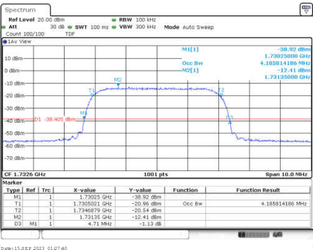
Band4-1413-4
