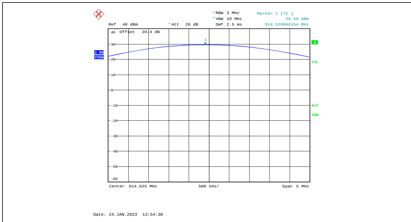
Plot 5.1.4.2. Maximum Peak Conducted Output Power, High Power, 230400 kbps, 914.625 MHz
