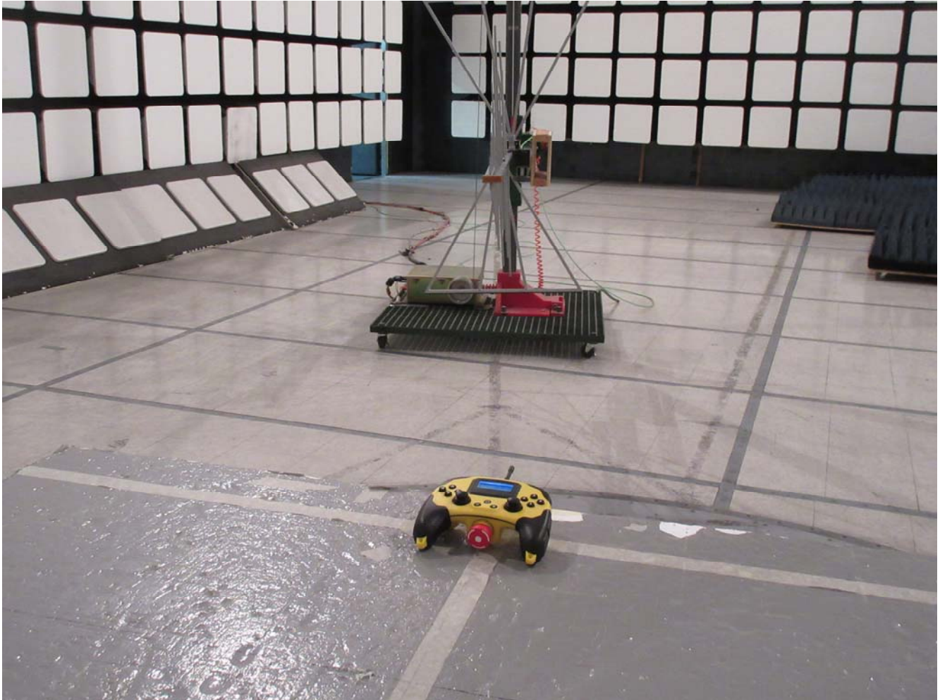
Radiated Emissions at 3 m EUT with 1.6 dBi Linx Technologies Inc ¼ wave whip, straight antenna, Orthogonal Position 1
