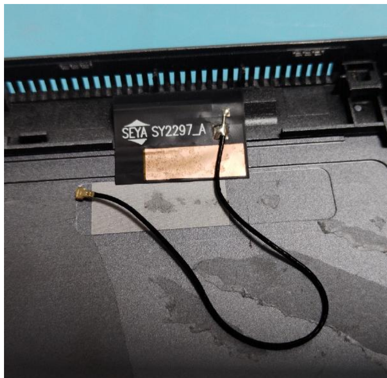
Wi-Fi ANT2 & BT ANT
