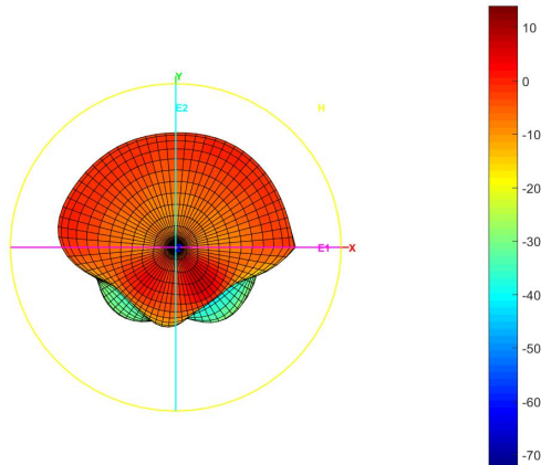
Total_3D_H_2.45GHz
