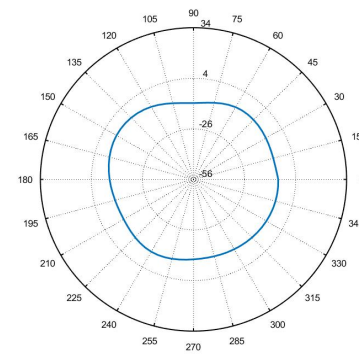
Total_Polar_H_2.45GHz
