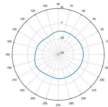
Total_Polar_E2_2.45GHz
