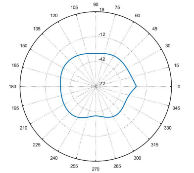
Total_Polar_E2_2.45GHz
