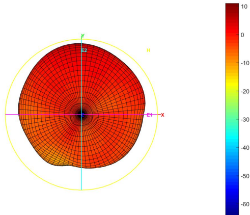
Total_3D_H_5.5GHz
