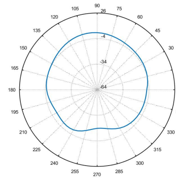
Total_Polar_H_5.5GHz
