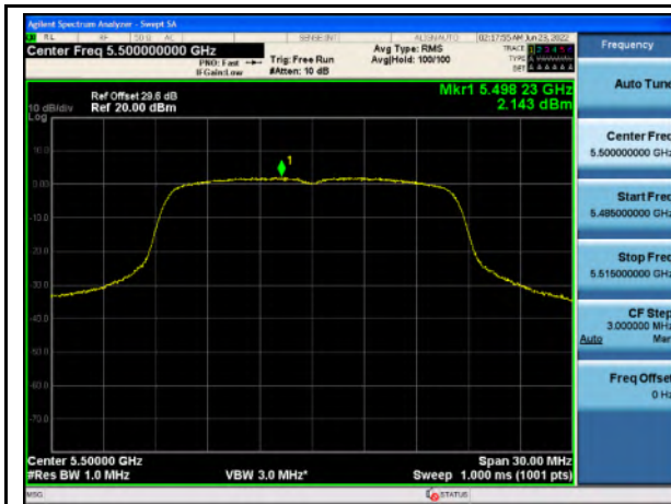
PSD_U-NII-2C_802.11a_5500
