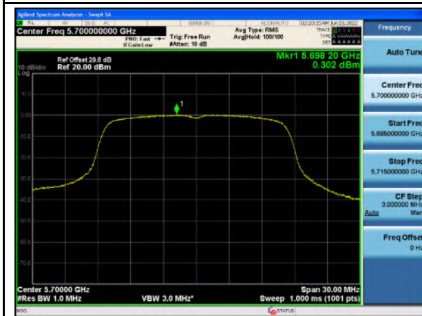
PSD_U-NII-2C_802.11a_5700
