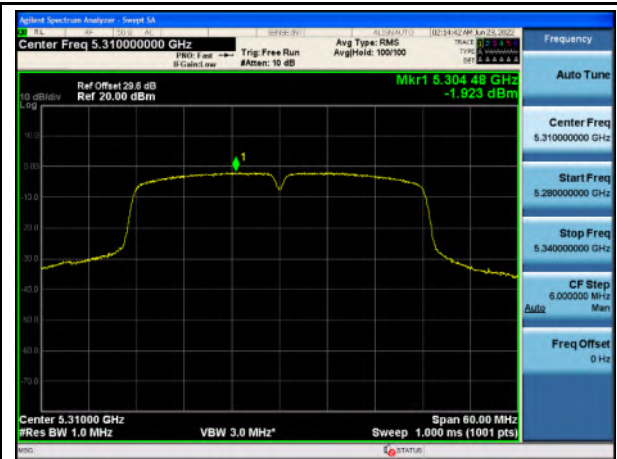
PSD_U-NII-2A_802.11n40_5310
