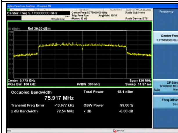
6 dB & 99% BW_U-NII-3_802.11ac80_5775
