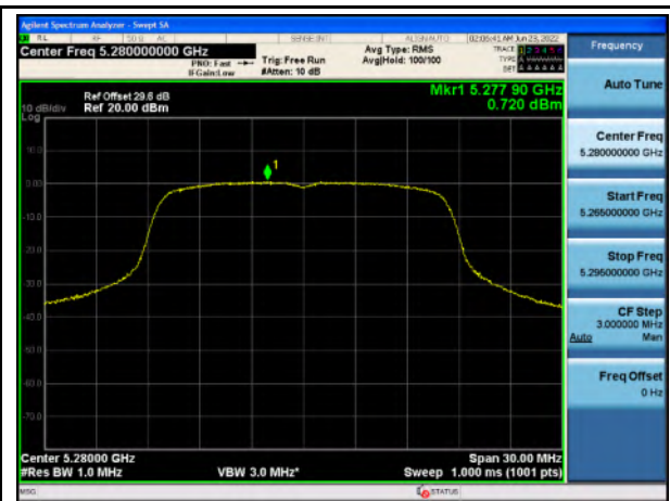
PSD_U-NII-2A_802.11a_5280
