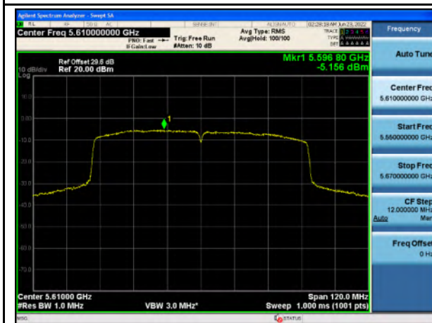
PSD_U-NII-2C_802.11ac80_5610
