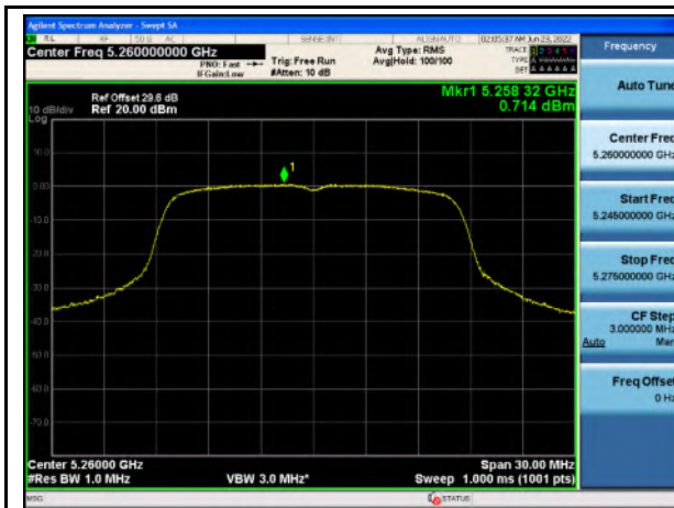
PSD_U-NII-2A_802.11a_5260
