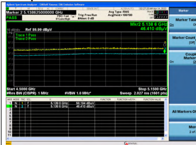
Restricted Band -11a-5180MHz
