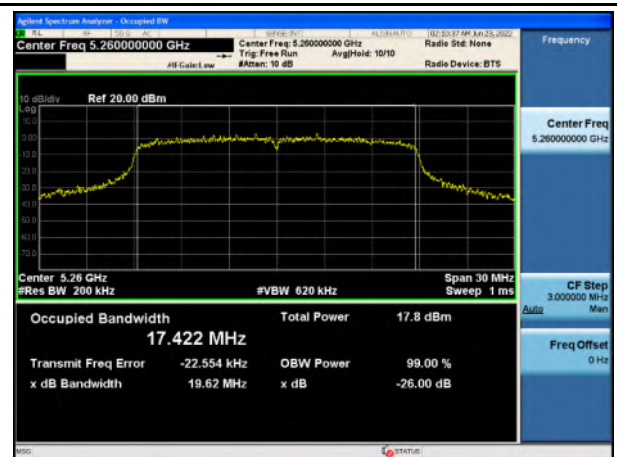
26 dB & 99% BW_U-NII-2A_802.11n_5260
