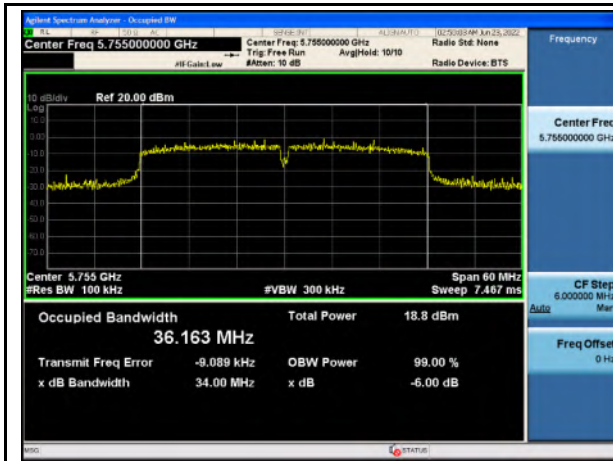
6 dB & 99% BW_U-NII-3_802.11n40_5755
