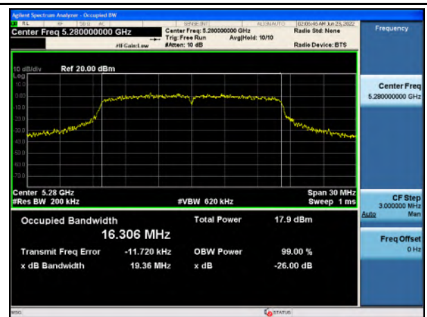
26 dB & 99% BW_U-NII-2A_802.11a_5280
