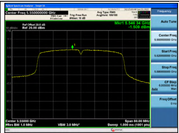
PSD_U-NII-2C_802.11n40_5550
