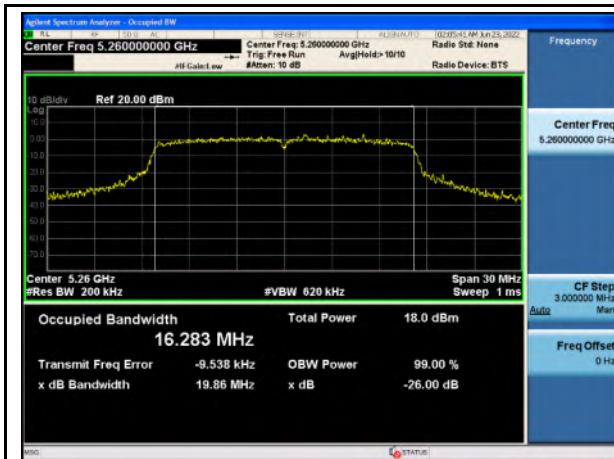
26 dB & 99% BW_U-NII-2A_802.11a_5260
