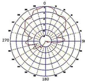
Element 3: Typical E Plane Pattern
