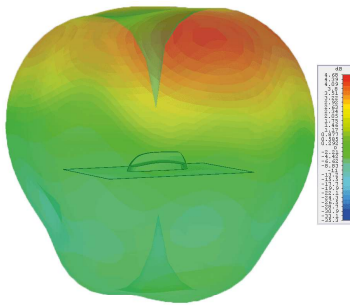
3D Gain Plot Top (800MHz)
