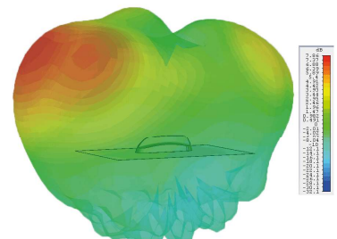
3D Gain Plot Side (2100MHz)
