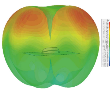
3D Gain Plot Top (1800MHz)
