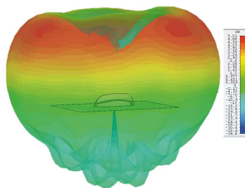
3D Gain Plot Side (1800MHz)
