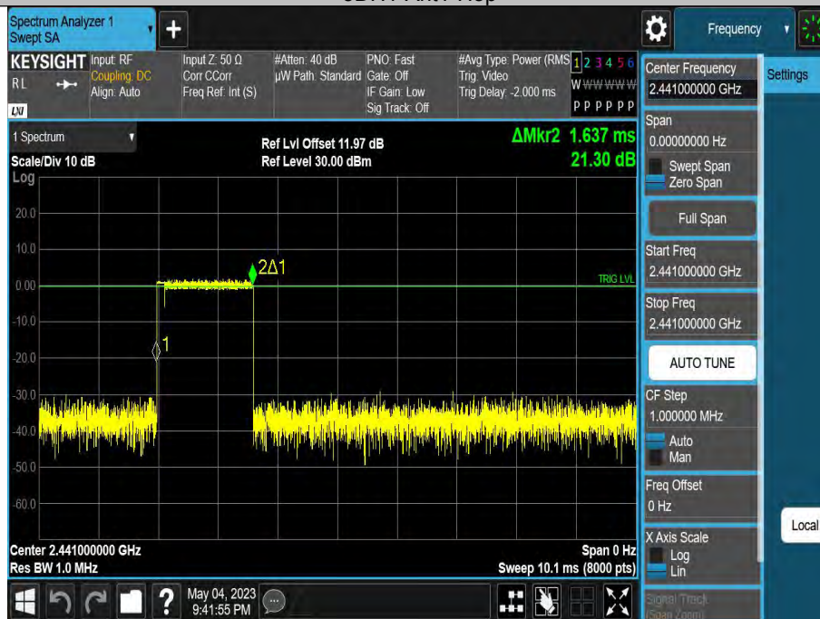
3DH3-Ant1-Hop
