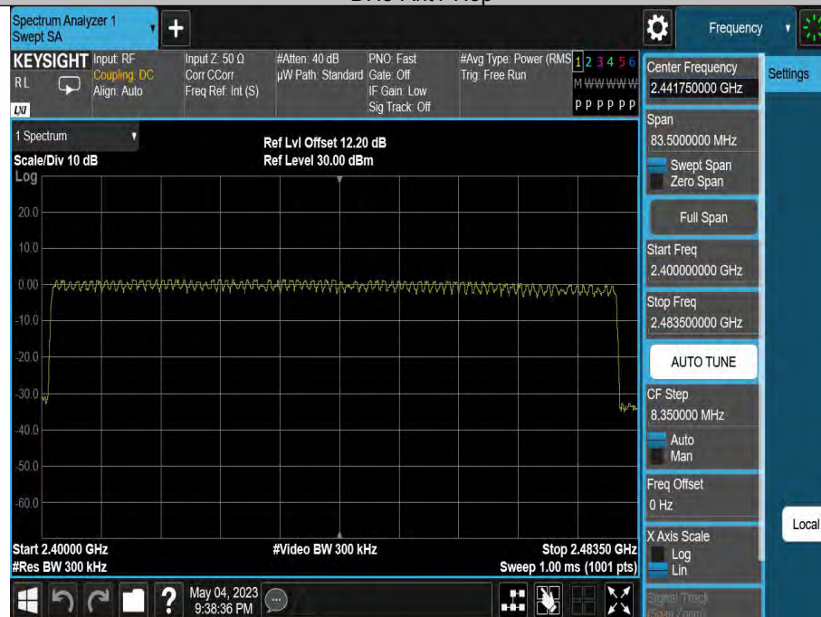
2DH5-Ant1-Hop
