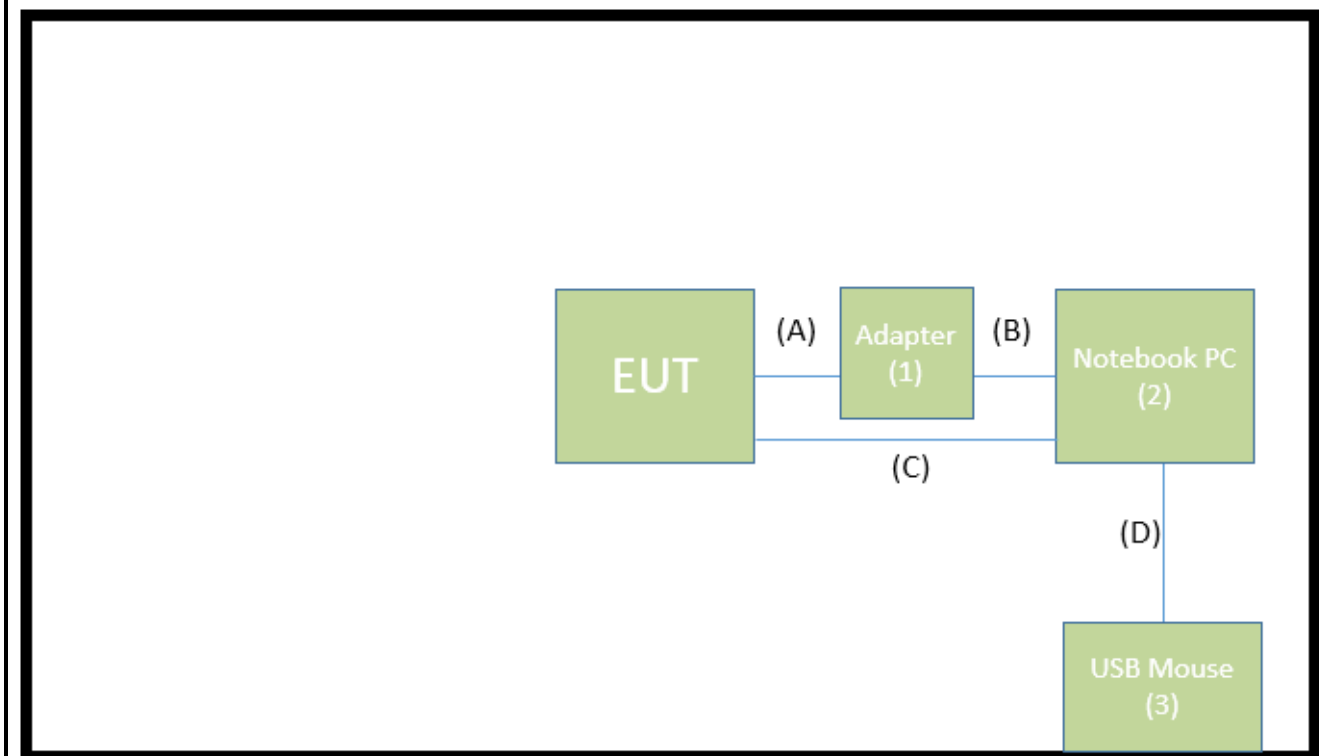
Connection Diagram
