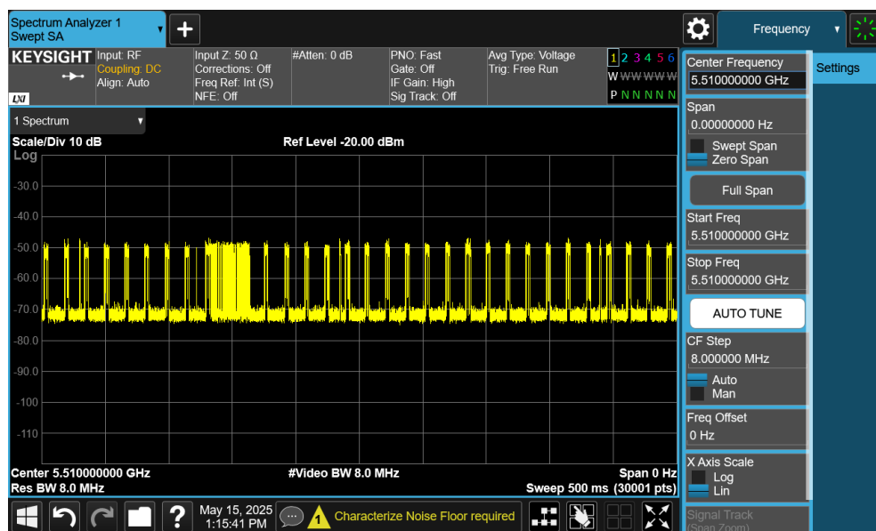
Channel Loading Plot - 802.11ac40-5510MHz
