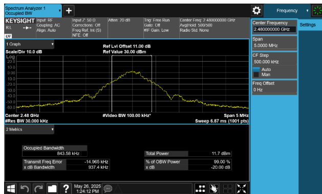
CH39 (2480MHz) 3-DH5(3Mbps)
