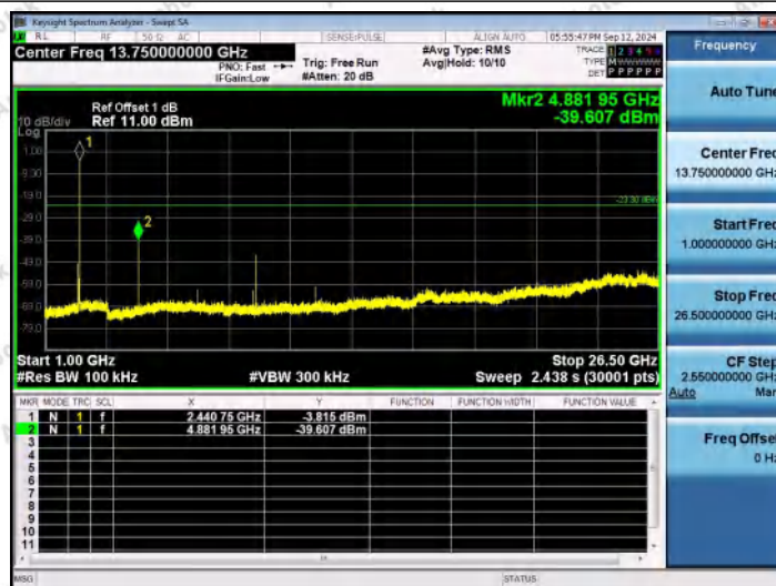
3DH5-Ant1-2441-1000~26500-PASS
