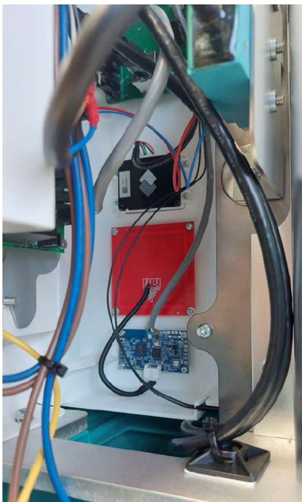
Detail, Barcode reader, RFID antenna and PCBA assembled in D45 - display housing.
