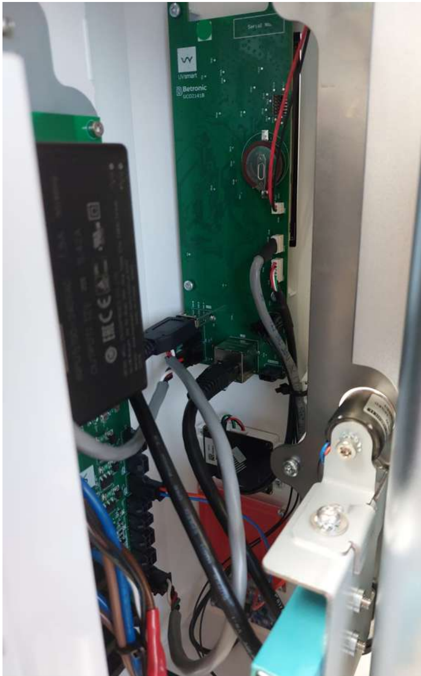
Detail: Control PCBA and Power PCBA
