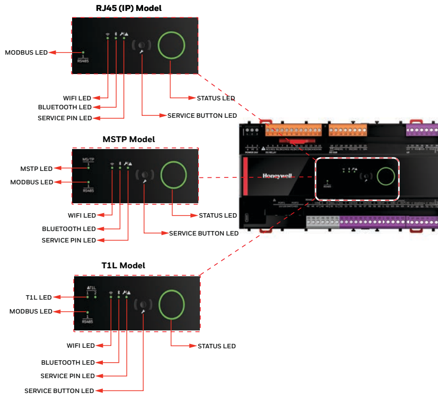
Figure 19. LED interface
