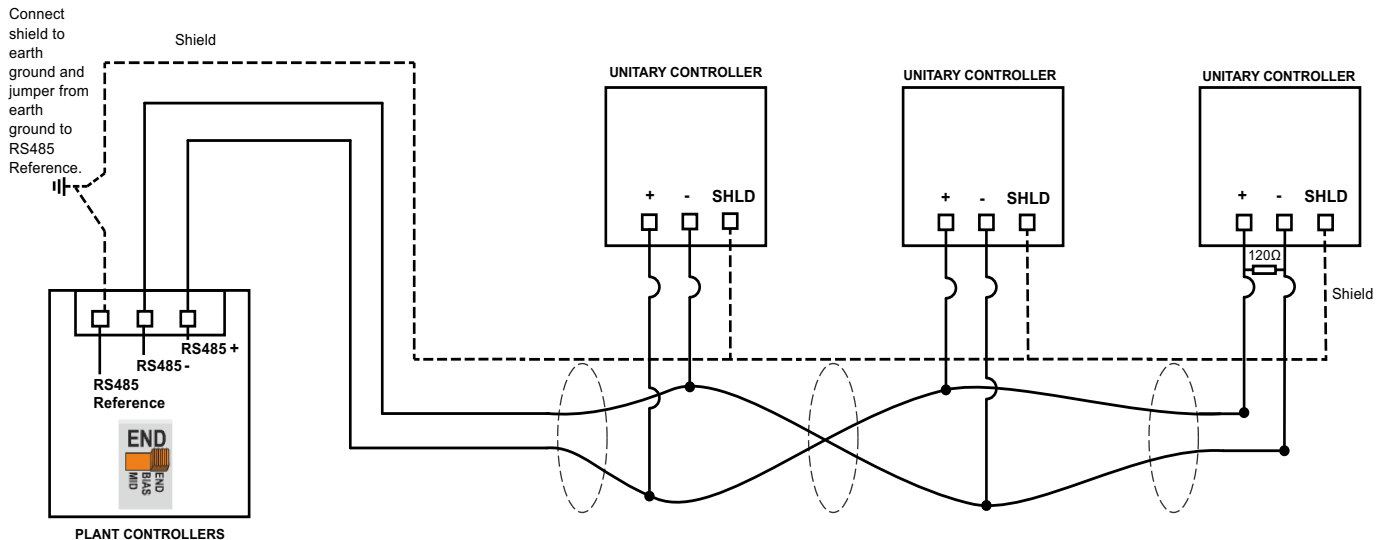
Figure 11. Connection to a BACnet™ MSTP Bus
