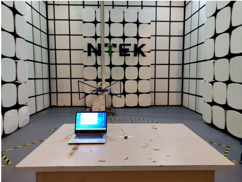
Radiated Measurement Photos(X-C13SG)
