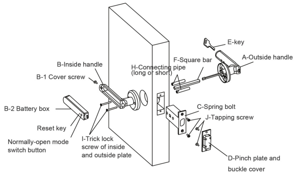
Diagram of Door Lock Installation
