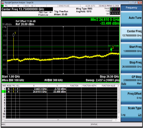
11N40SISO-Ant1-2452-1000~26500-PASS
