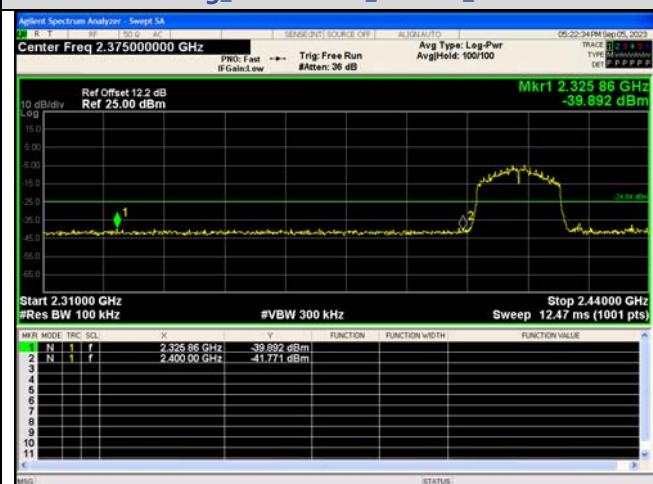
Out Of Band Emission IEEE 802.11n_Channel 1_20MHz_Antenna 0
