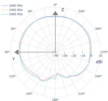
Model ANT-M2458-CBT02 Antenna Radiation Patterns at 2G4
