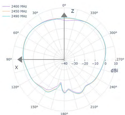
Model ANT-M2458-CBT03 Antenna Radiation Patterns at 2G4
