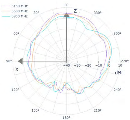
Model ANT-M2458-CBT03 Antenna Radiation Patterns at 5G
