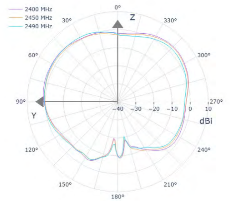
Model ANT-M2458-CBT04 Antenna Radiation Patterns at 2G4
