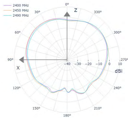
Model ANT-M2458-CBT04 Antenna Radiation Patterns at 2G4
