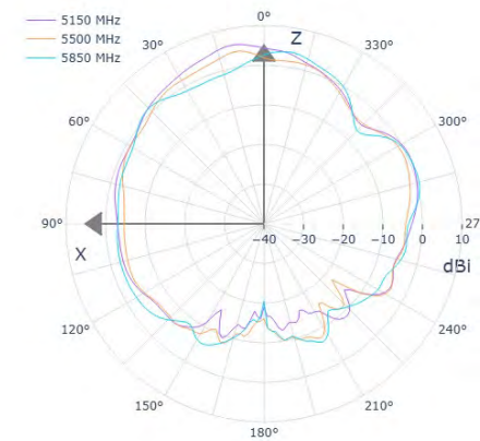
Model ANT-M2458-CBT04 Antenna Radiation Patterns at 5G
