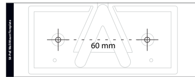
Horizontal Mount
