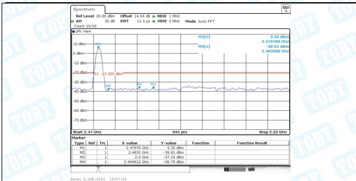
DH5_Ant1_High_2480_Peak
