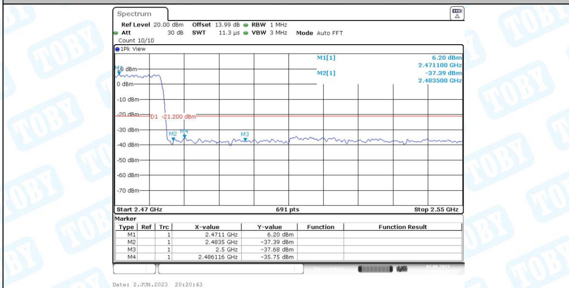
2DH5_Ant1_High_Hop_2480_Peak
