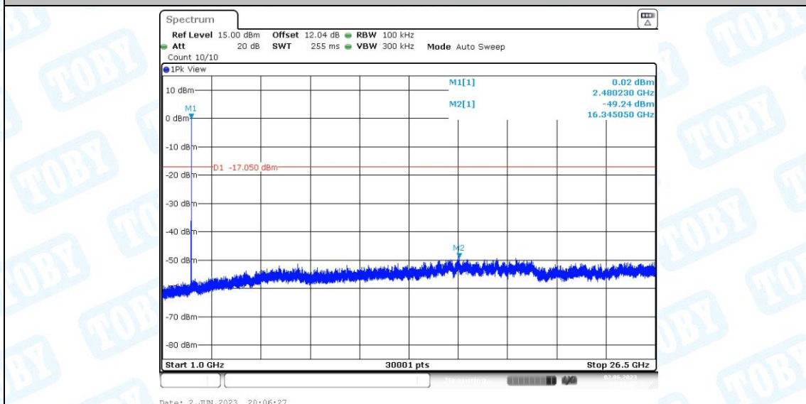
2DH5_Ant1_2480_1000~26500
