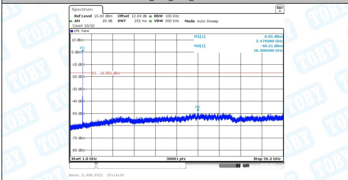
3DH5_Ant1_2480_1000~26500
