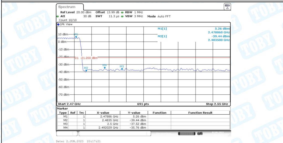
DH5_Ant1_High_Hop_2480_Peak
