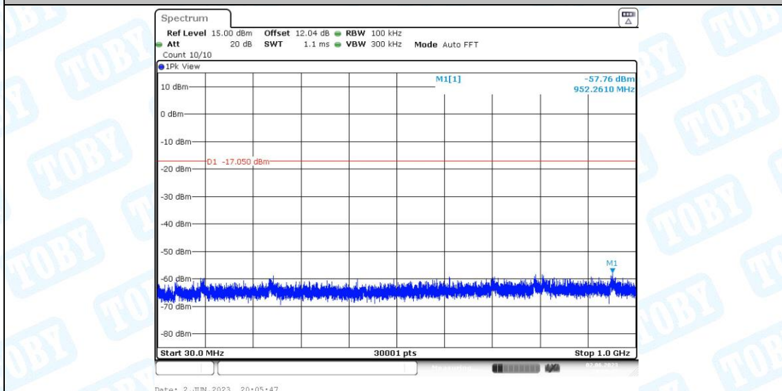
2DH5_Ant1_2480_30~1000
