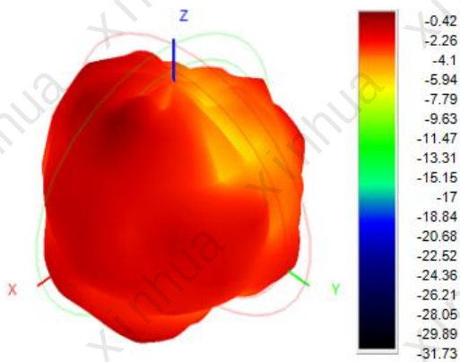
(4) 2400.0MHz H+V, Eff: 26.5%
