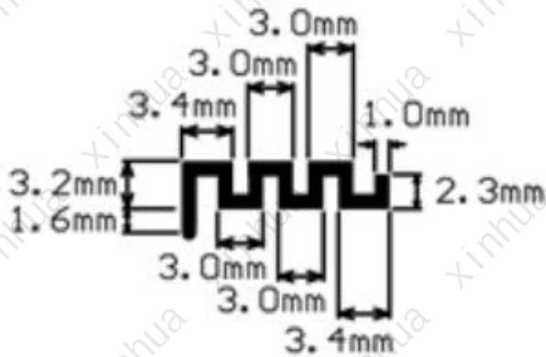
Antenna Dimensions
