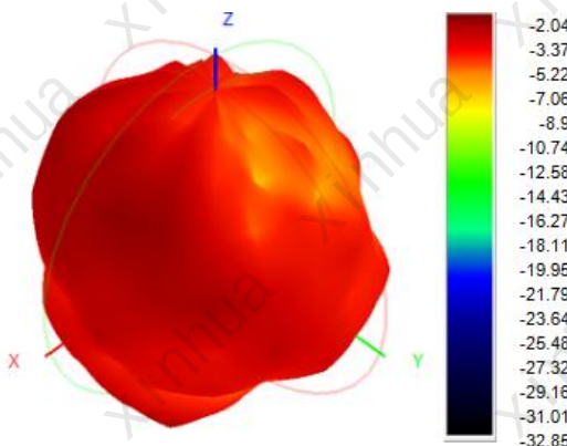
(6) 2500.0MHz H+V, Eff: 25.7%
