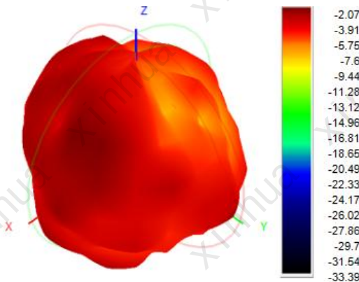
(5) 2450.0MHz H+V, Eff: 22.7%
