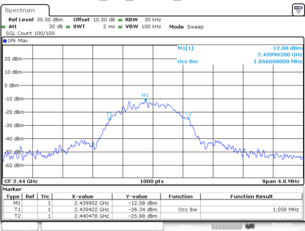
BLE_1M_Middle_Channel
