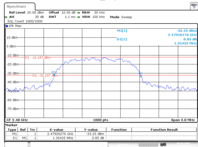
3DH5_High
