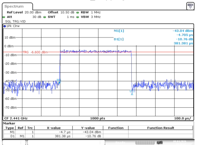
3DH1_Hopping
