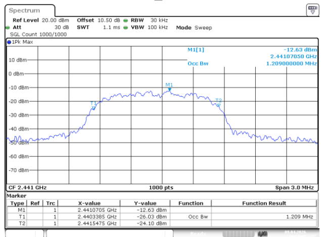
3DH5_Middle
