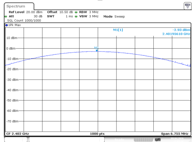
3DH5_Low
