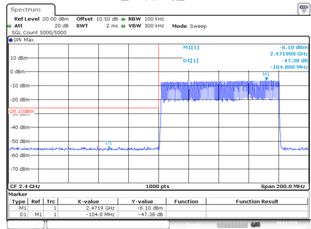
DH5_Hopping_Lower
