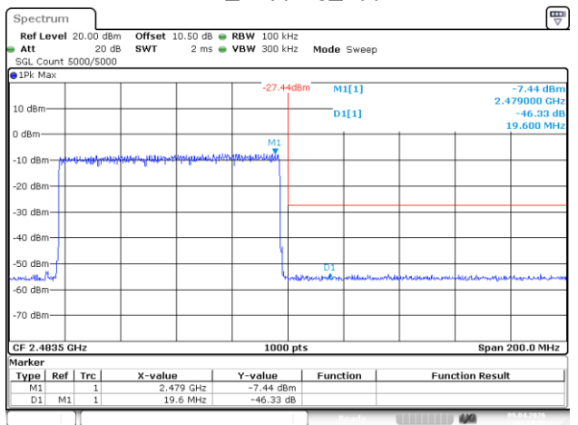
3DH5_Hopping_Upper
