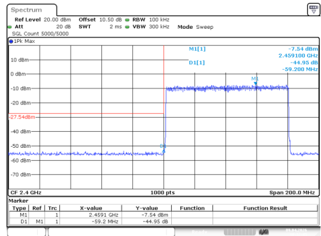
2DH5_Hopping_Lower
