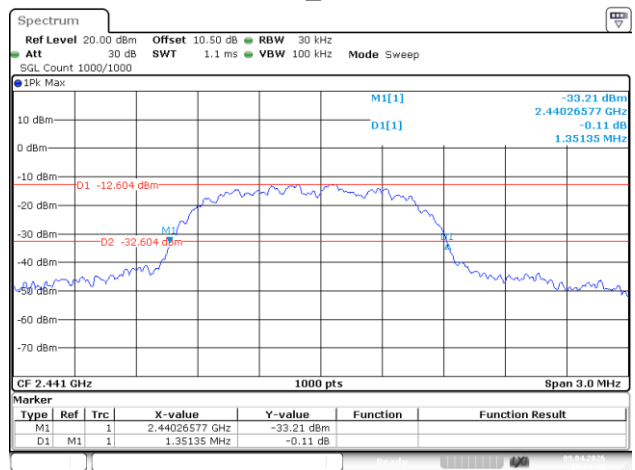
3DH5_Middle
