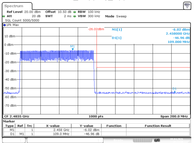
DH5_Hopping_Upper
