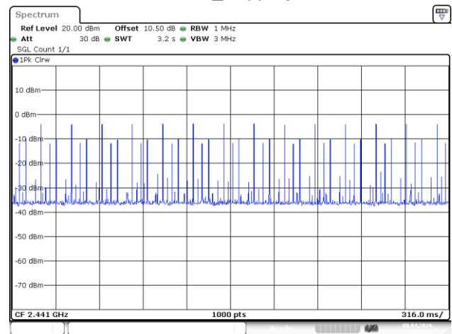
3DH3_Hopping
