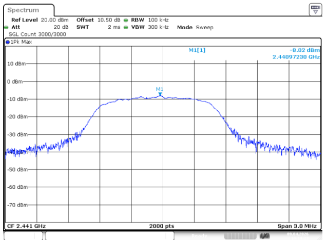
2DH5_Middle
