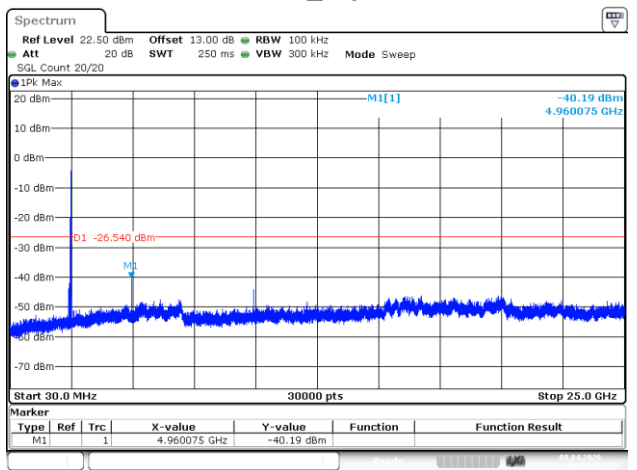
DH5_High
