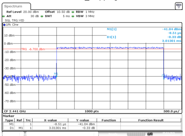
3DH5_Hopping
