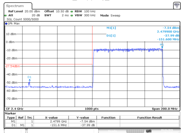
3DH5_Hopping_Lower
