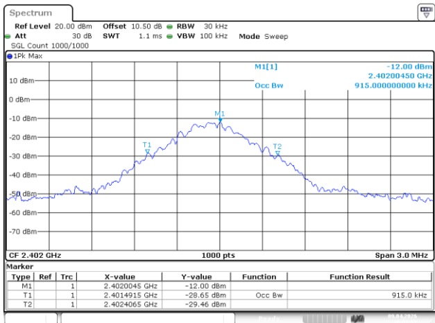
DH5_Low
