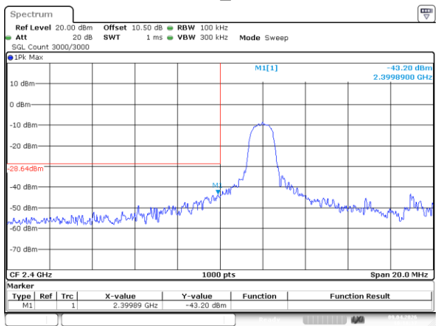
2DH5_Low
