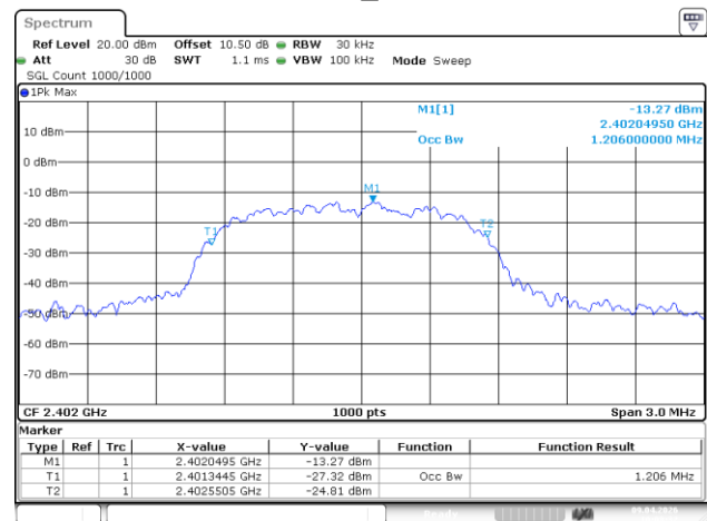
3DH5_Low
