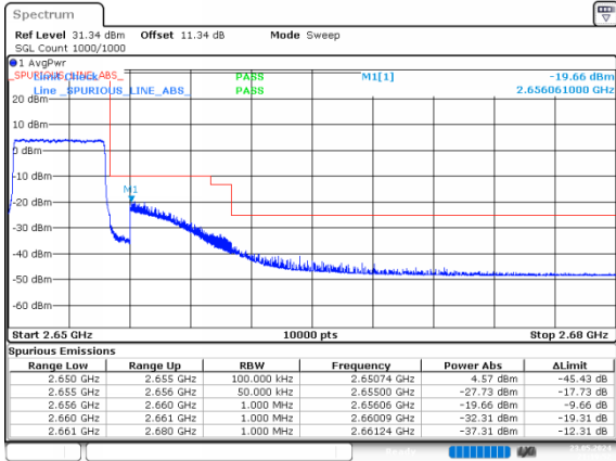
2_5MHz_High_16QAM_25@0
