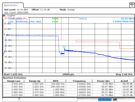
2_20MHz_High_16QAM_100@0
