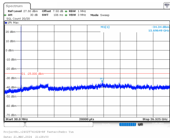
2_10MHz_Middle_QPSK_1@0
