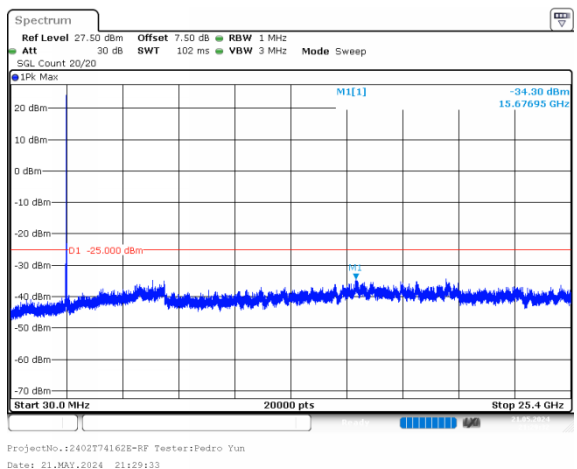
2_10MHz_High_QPSK_1@0
