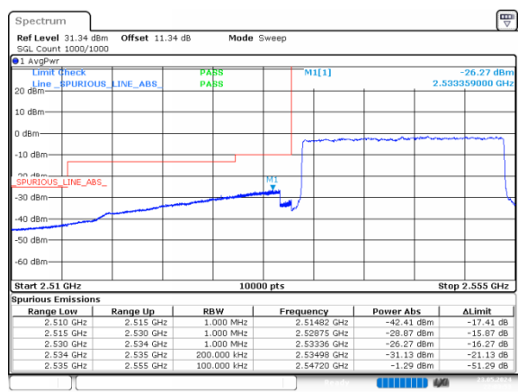
2_20MHz_Low_16QAM_100@0
