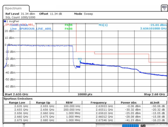
2_20MHz_High_QPSK_100@0
