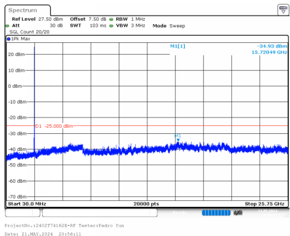
10MHz_High_QPSK_1@0
