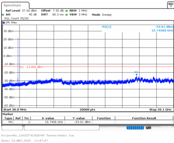
3MHz_High_QPSK_1@0
