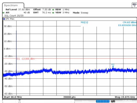
5MHz_High_QPSK_1@0
