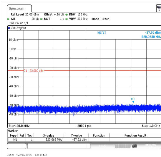
Band4-3MHz-QPSK-20175-1RB#0-30~1000-PAS
