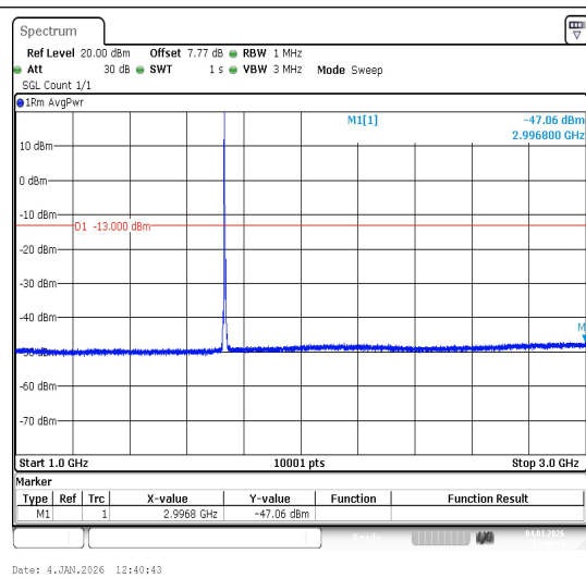
Band4-3MHz-QPSK-20175-1RB#0-1000~3000-PA
