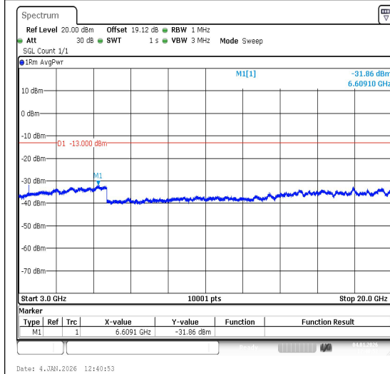
Band4-3MHz-QPSK-20175-1RB#0-3000~20000-PASS
