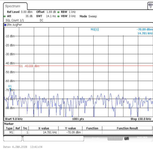
Band4-3MHz-16QAM-20175-1RB#0-0.009~0.15-PASS
