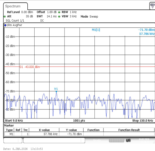
Band4-5MHz-16QAM-20175-1RB#0-0.009~0.15-P
