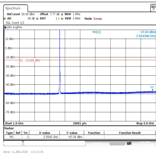
Band4-5MHz-QPSK-20175-1RB#0-1000~3000-PA
