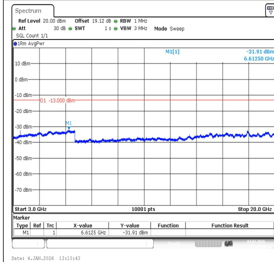
Band4-5MHz-QPSK-20175-1RB#0-3000~20000-
