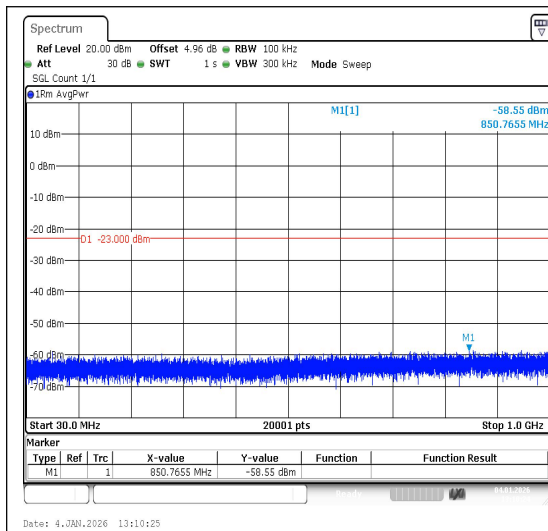
Band4-5MHz-QPSK-20175-1RB#0-30~1000-PAS
