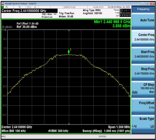
DH5-Ant1-2441-PASS
