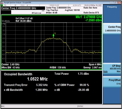
LE_1M-Ant1-2480
