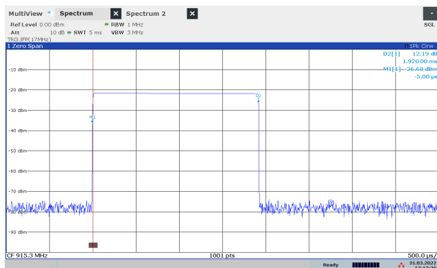
Burst Length
