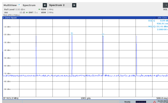
Burst Period
