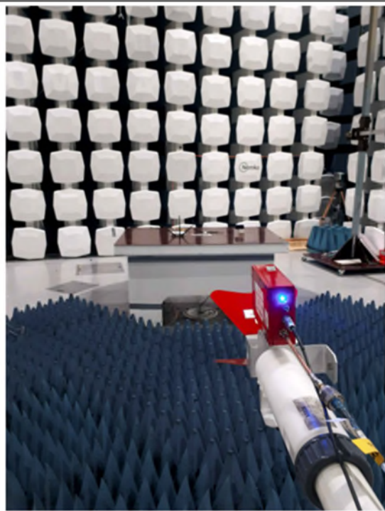
Radiated 1000 – 6000 MHz from antenna
