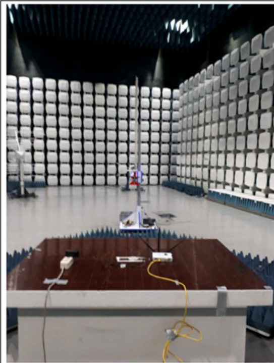
Radiated 1000 – 6000 MHz from EUT
