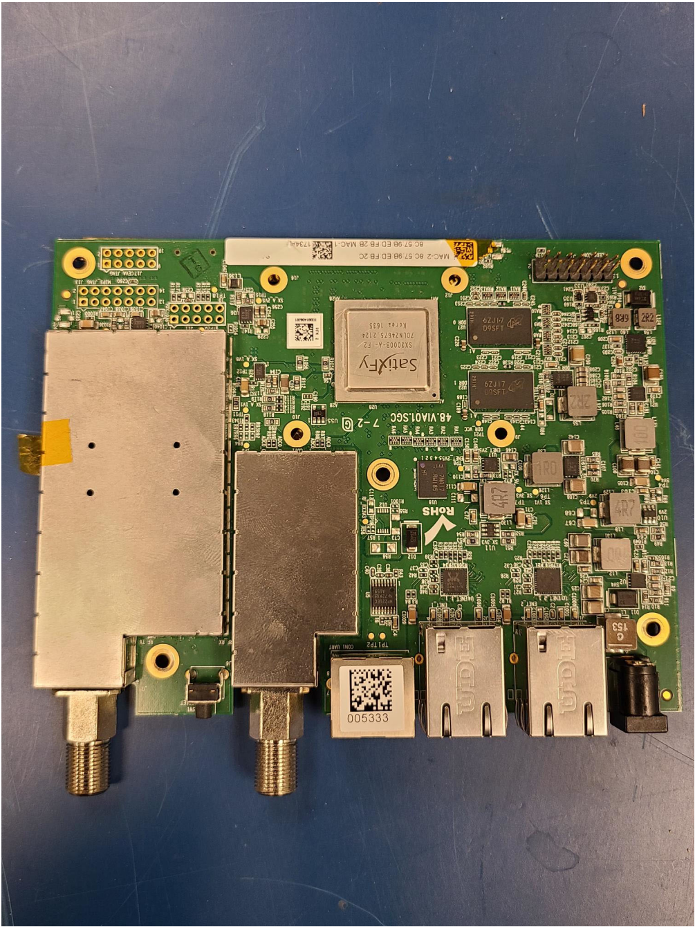
IQ200 Front
