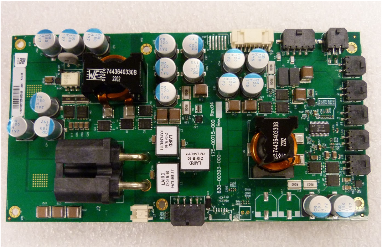
PSU Front
