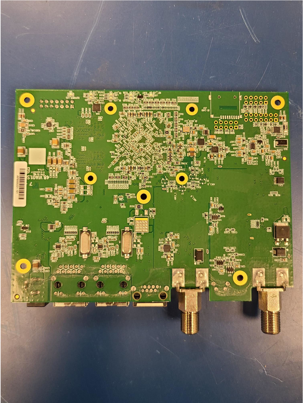
IQ200 Back
