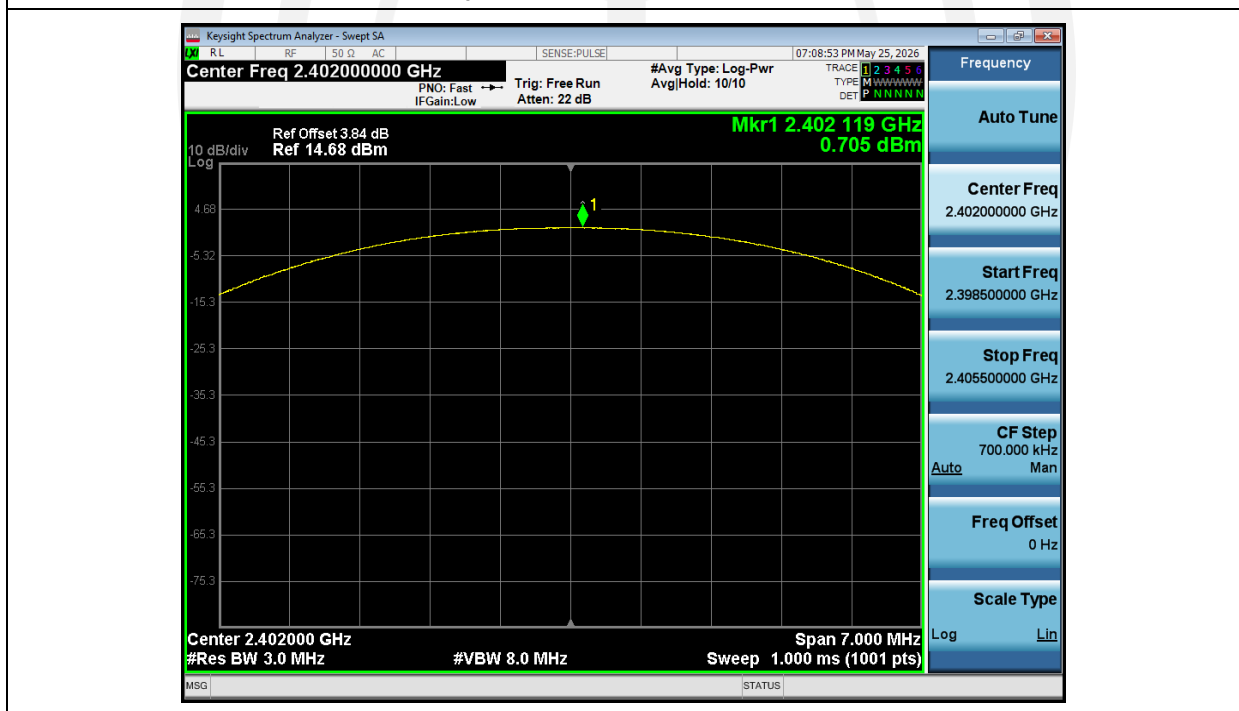
Peak_Output_Power_NVNT_ANT1_2-DH1_2402_00
