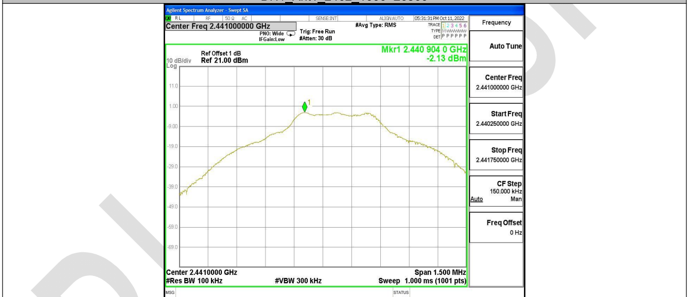
DH1_Ant1_2441_0~Reference
