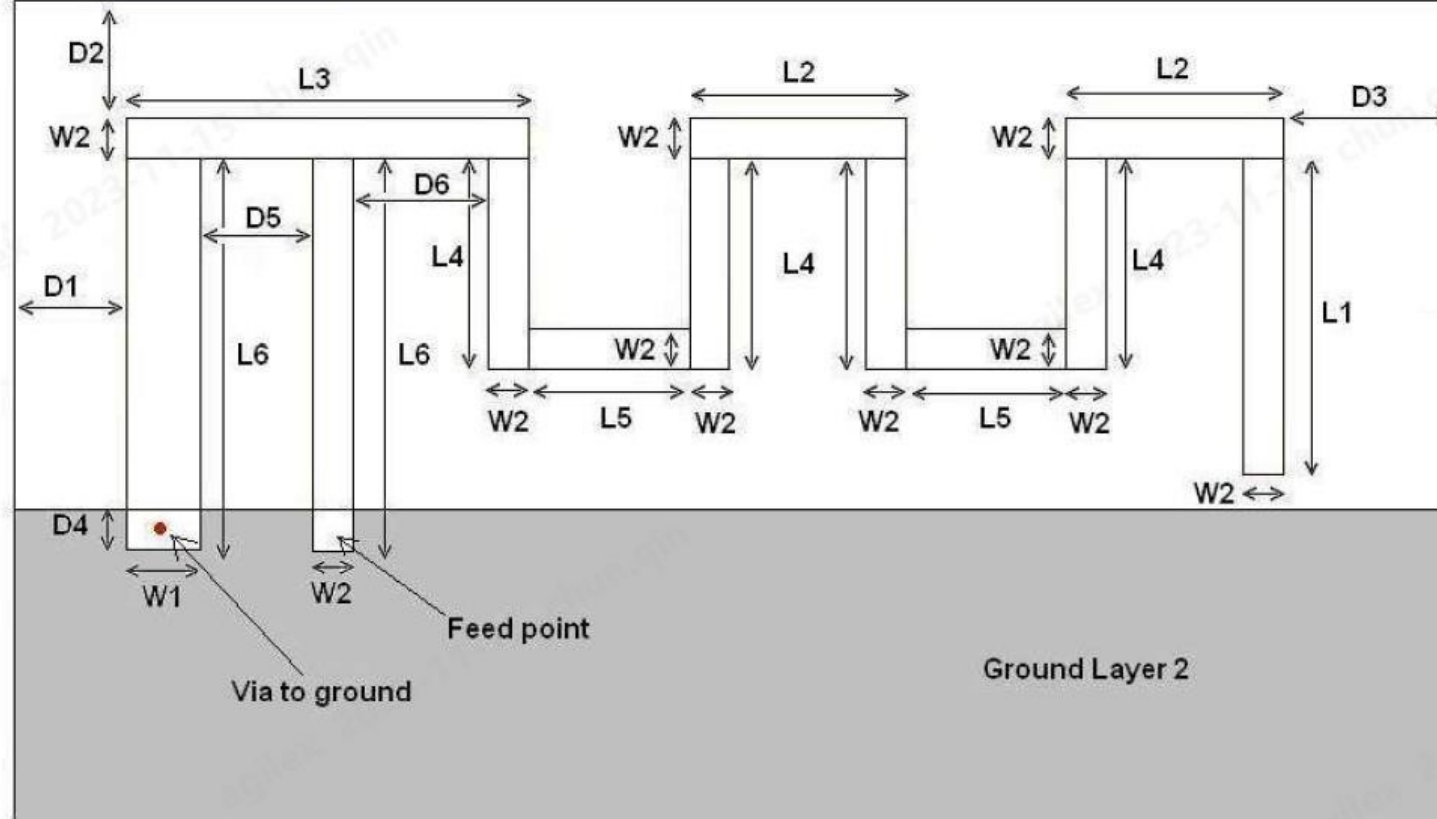
Figure 3: Antenna Dimensions
