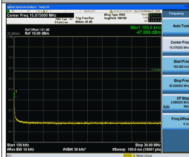
GPRS850-190-5-0.15~30MHz-PASS
