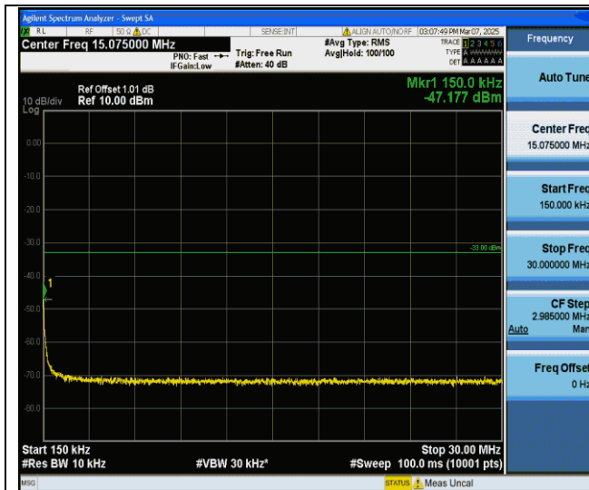
EGPRS1900-661-2-0.15~30MHz-PASS
