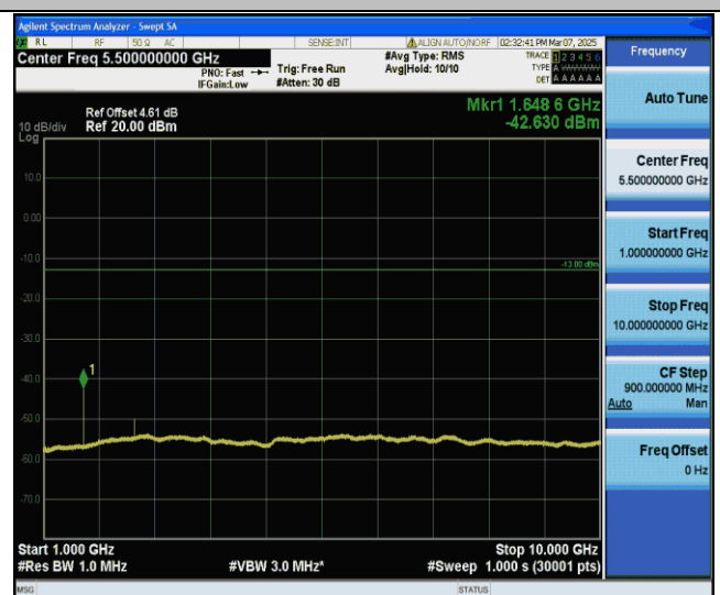
EGPRS850-128-8-1000~10000MHz-PASS
