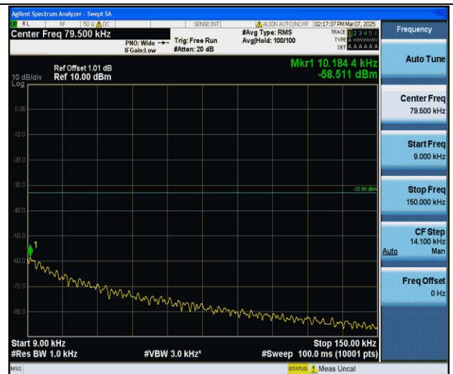
GPRS850-190-5-0.009~0.15MHz-PASS
