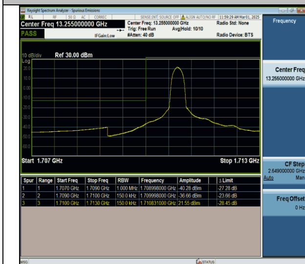
Band4-15MHz-QPSK-20025-1RB#0-PASS
