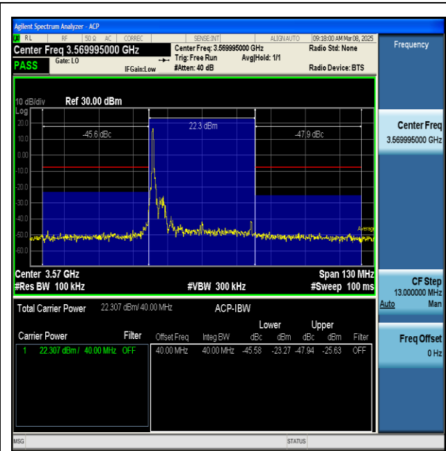
NTVN-n48-PC3-30-40-L-CP-QPSK-Inner_1RB_Left-PASS
