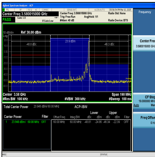
NTNV-n48-PC3-30-60-L-DFT-BPSK-Inner_1RB_Right- PASS
