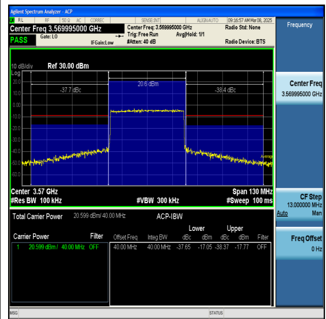
NTNV-n48-PC3-30-40-L-CP-QPSK-Outer_Full-PASS
