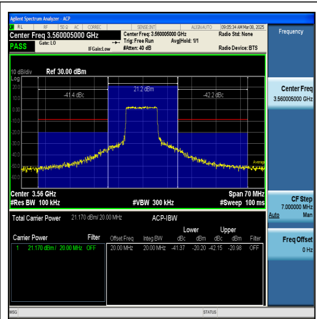
NTNV-n48-PC3-30-20-L-CP-QPSK-Inner_Full-PASS
