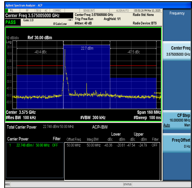
NTNV-n48-PC3-30-50-L-DFT-BPSK-Inner_1RB_Left- PASS
