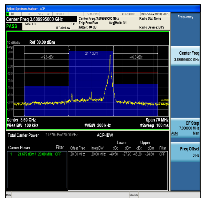
NTNV-n48-PC3-30-20-H-CP-QPSK-Inner_1RB_Right-PASS
