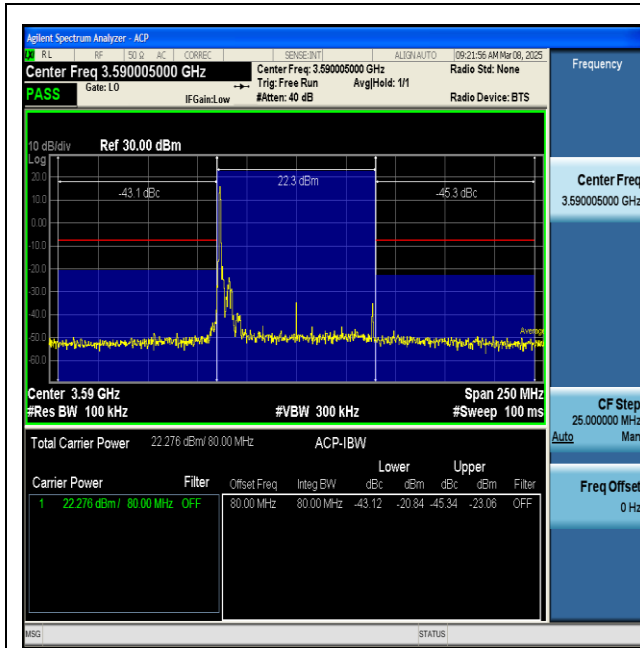
NTNV-n48-PC3-30-80-L-DFT-BPSK-Inner_1RB_Left- PASS
