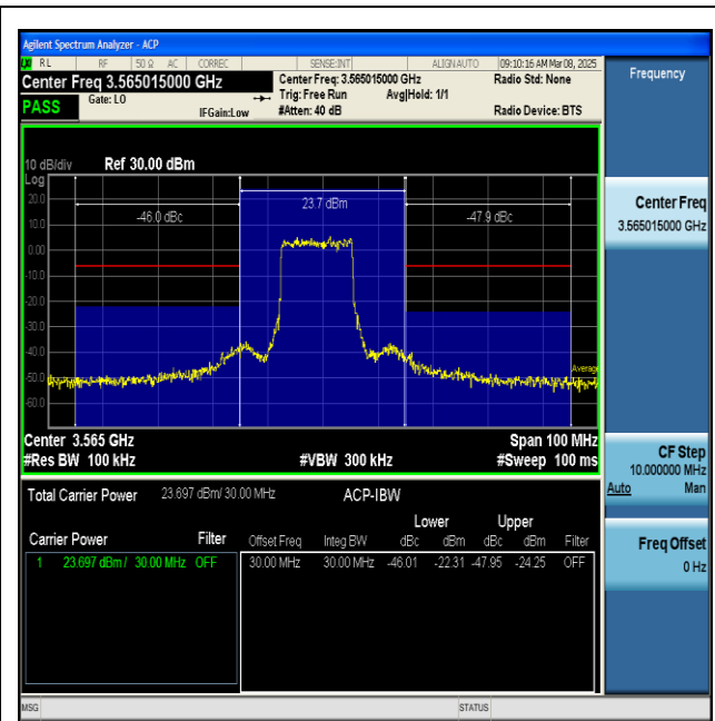
NTNV-n48-PC3-30-30-L-DFT-BPSK-Inner_Full-PASS
