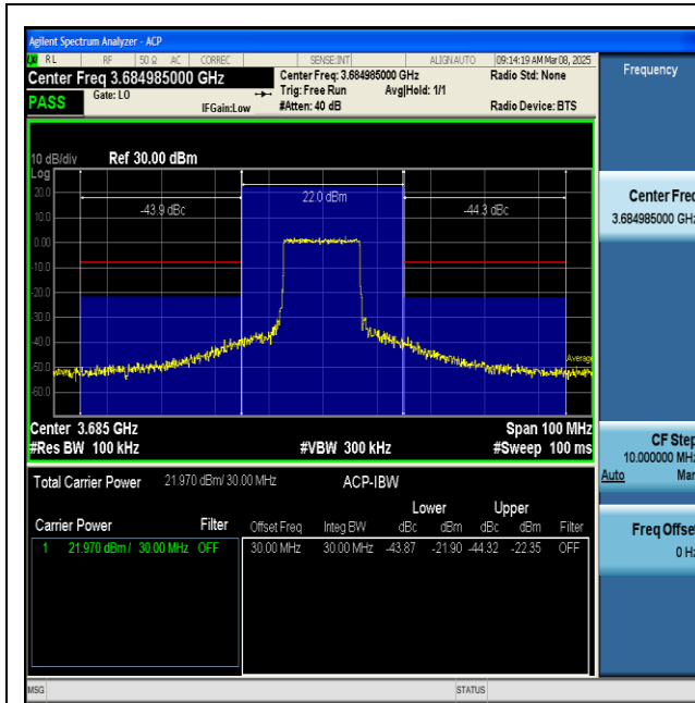
NTNV-n48-PC3-30-30-H-CP-QPSK-Inner_Full-PASS
