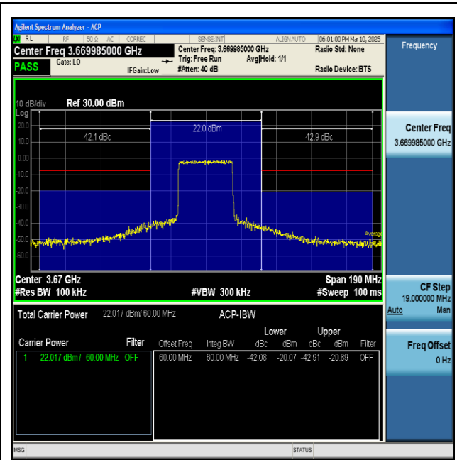
NTNV-n48-PC3-30-60-H-CP-QPSK-Inner_Full-PASS
