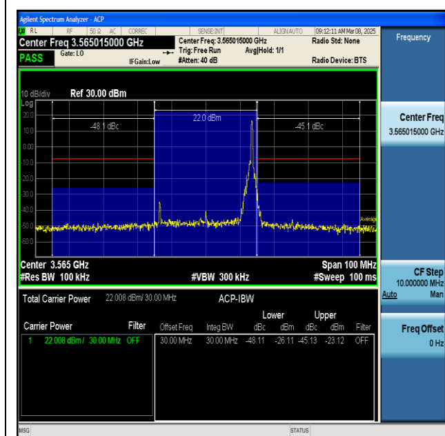
NTNV-n48-PC3-30-30-L-CP-QPSK-Inner_1RB_Right-PASS
