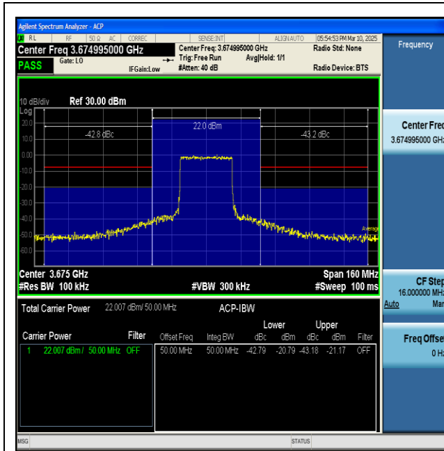
NTNV-n48-PC3-30-50-H-CP-QPSK-Inner_Full-PASS
