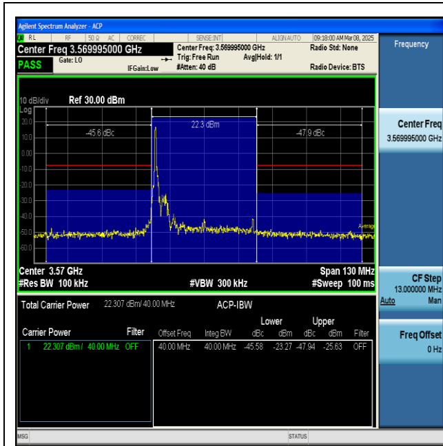
NTVN-n48-PC3-30-40-L-CP-QPSK-Inner_1RB_Left-PASS
