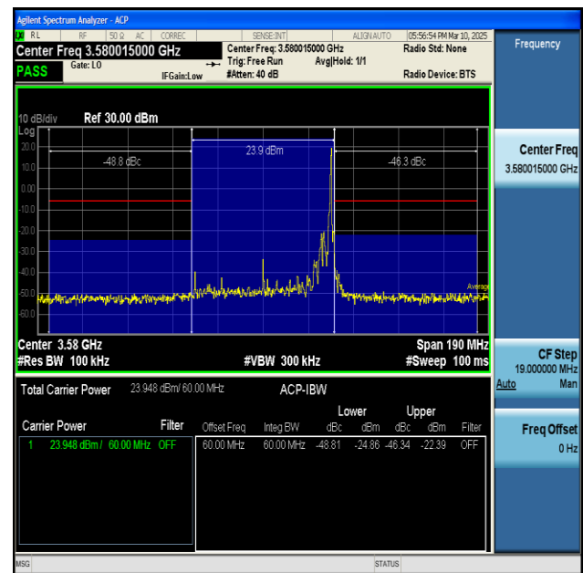
NTNV-n48-PC3-30-60-L-DFT-BPSK-Inner_1RB_Right- PASS
