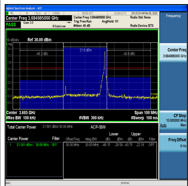
NTNV-n48-PC3-30-30-H-CP-QPSK-Inner_1RB_Right-PASS
