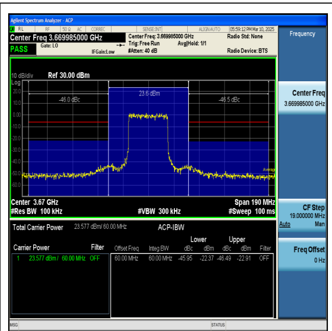
NTNV-n48-PC3-30-60-H-DFT-BPSK-Inner_Full-PASS
