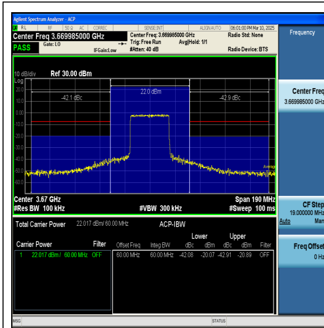
NTNV-n48-PC3-30-60-H-CP-QPSK-Inner_Full-PASS
