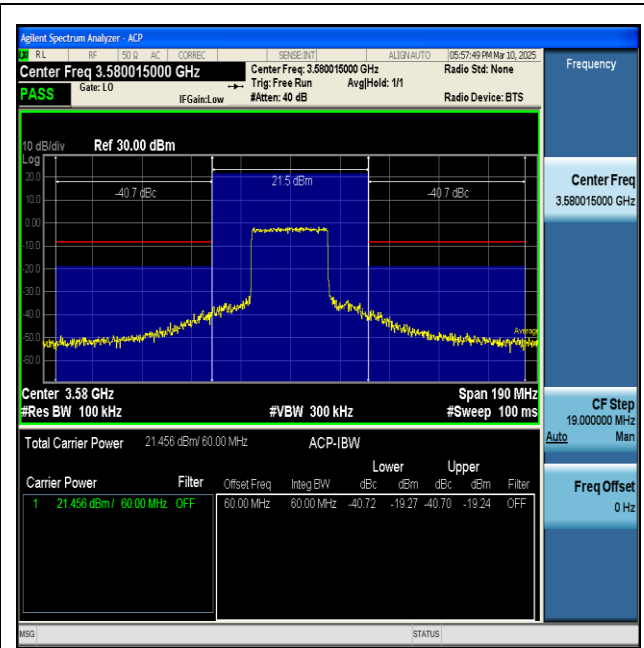
NTNV-n48-PC3-30-60-L-CP-QPSK-Inner_Full-PASS
