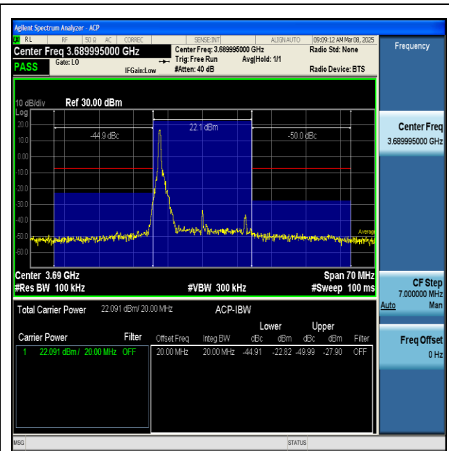
NTNV-n48-PC3-30-20-H-CP-QPSK-Inner_1RB_Left-PASS
