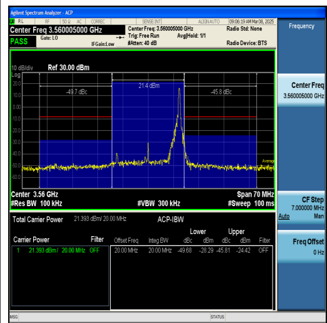
NTVN-n48-PC3-30-20-L-CP-QPSK-Inner_1RB_Right-PASS
