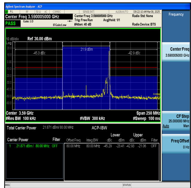
NTNV-n48-PC3-30-80-L-DFT-BPSK-Inner_1RB_Right- PASS
