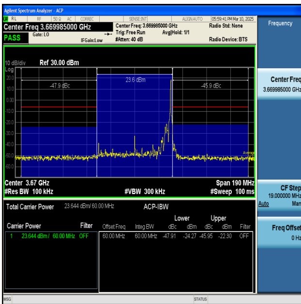
NTNV-n48-PC3-30-60-H-DFT-BPSK-Inner_1RB_Right- PASS
