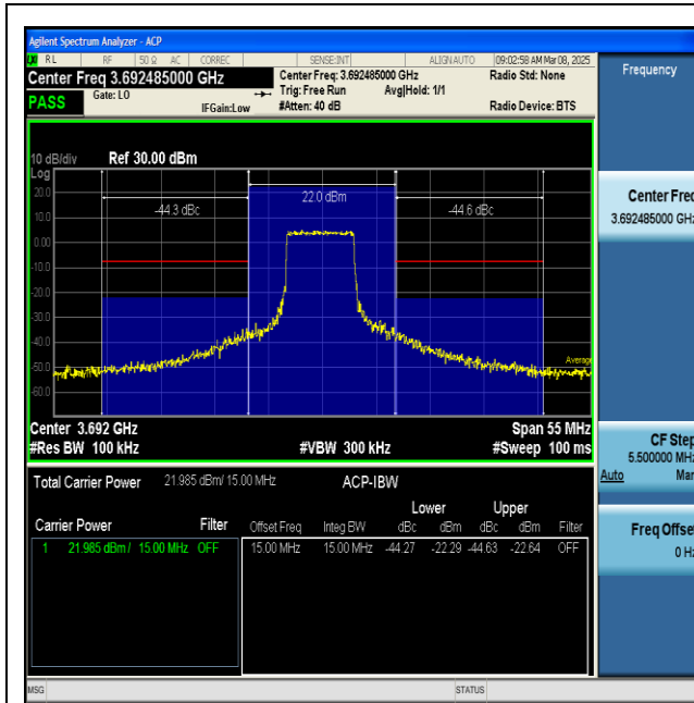
NTNV-n48-PC3-30-15-H-CP-QPSK-Inner_Full-PASS
