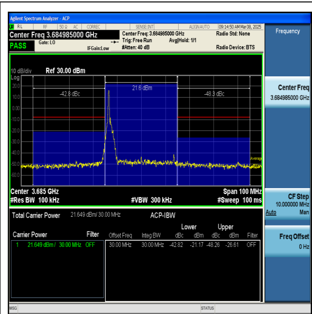
NTNV-n48-PC3-30-30-H-CP-QPSK-Inner_1RB_Left-PASS
