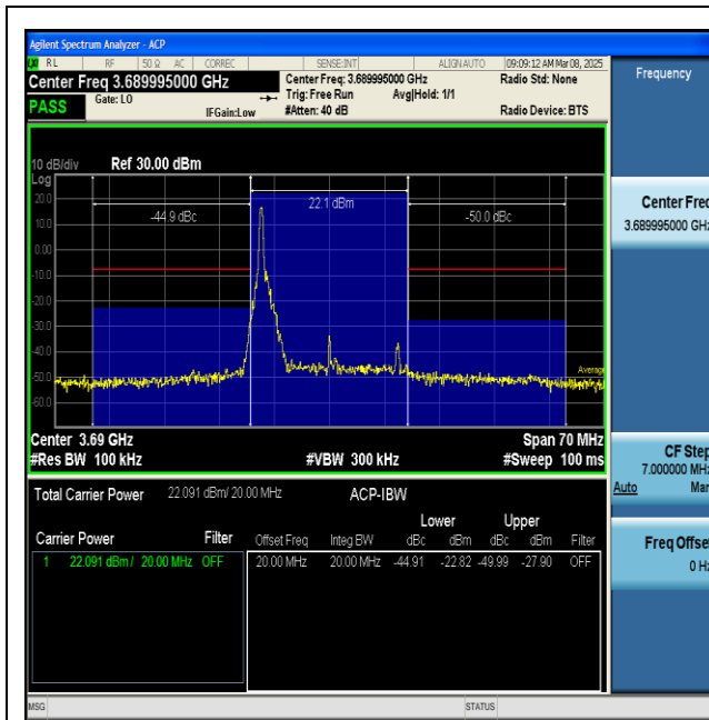
NTNV-n48-PC3-30-20-H-CP-QPSK-Inner_1RB_Left-PASS
