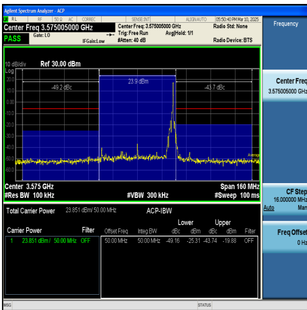
NTNV-n48-PC3-30-50-L-DFT-BPSK-Inner_1RB_Right- PASS
