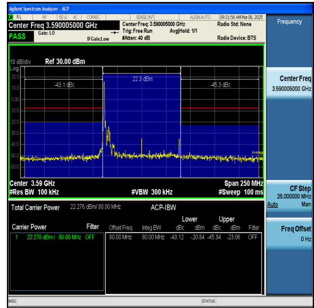
NTNV-n48-PC3-30-80-L-DFT-BPSK-Inner_1RB_Left- PASS
