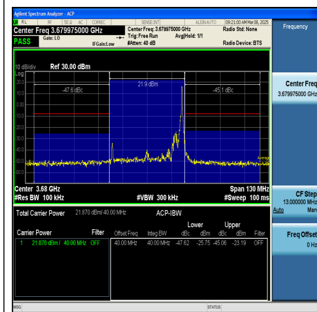
NTNV-n48-PC3-30-40-H-CP-QPSK-Inner_1RB_Right-PASS
