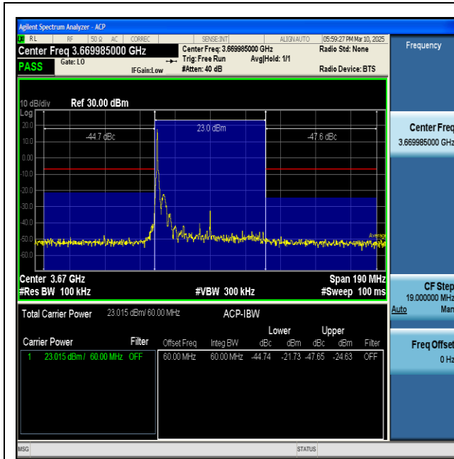
NTNV-n48-PC3-30-60-H-DFT-BPSK-Inner_1RB_Left- PASS
