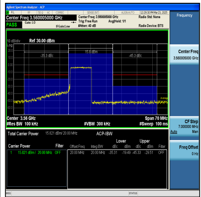
NTNV-n48-PC3-30-20-L-CP-QPSK-Outer_Full-PASS
