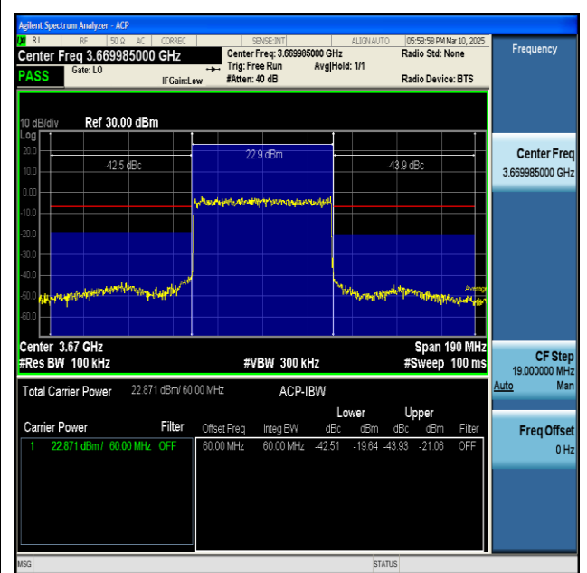
NTNV-n48-PC3-30-60-H-DFT-BPSK-Outer Full-PASS
