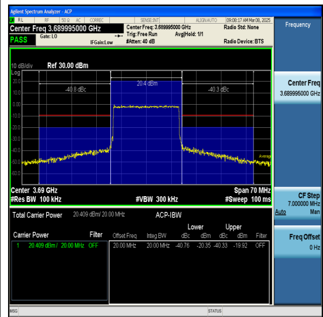
NTNV-n48-PC3-30-20-H-CP-QPSK-Outer_Full-PASS
