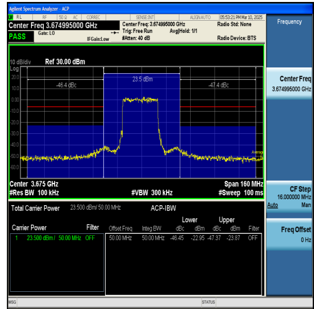
NTNV-n48-PC3-30-50-H-DFT-BPSK-Inner_Full-PASS
