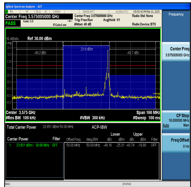
NTNV-n48-PC3-30-50-L-DFT-BPSK-Inner_1RB_Right- PASS
