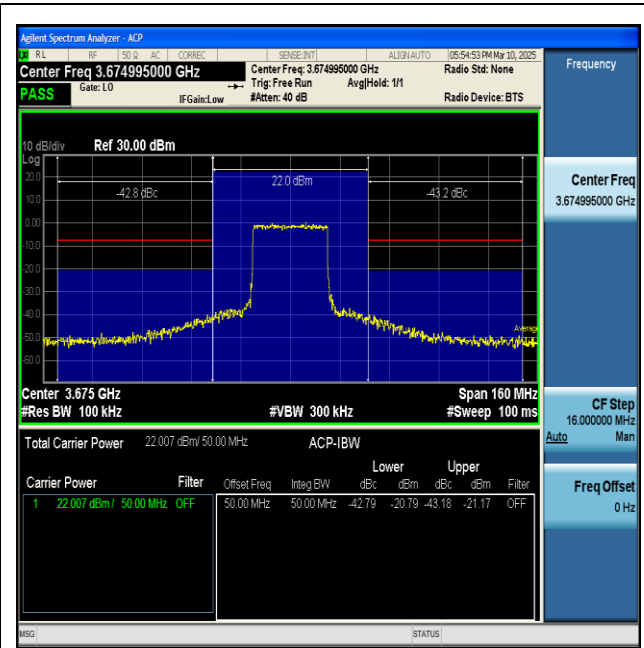
NTNV-n48-PC3-30-50-H-CP-QPSK-Inner_Full-PASS
