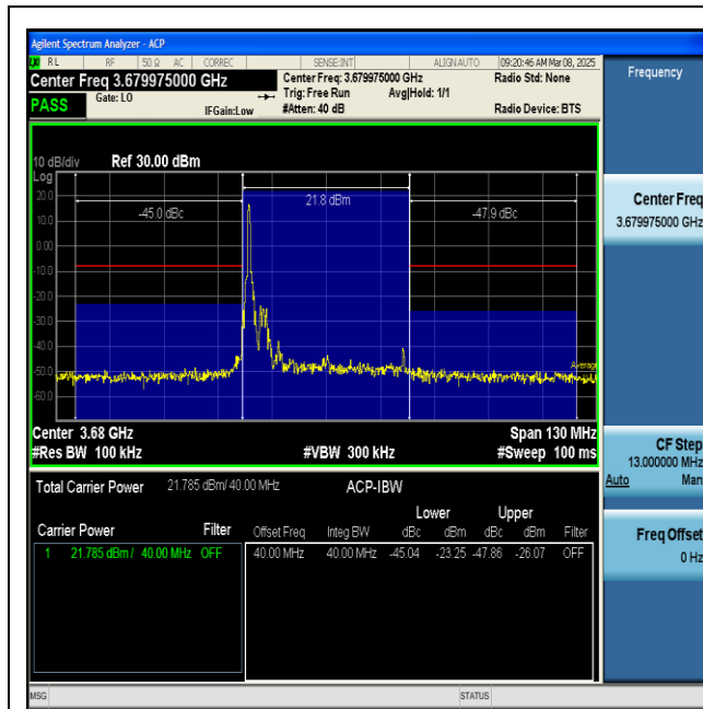
NTNV-n48-PC3-30-40-H-CP-QPSK-Inner_1RB_Left-PASS
