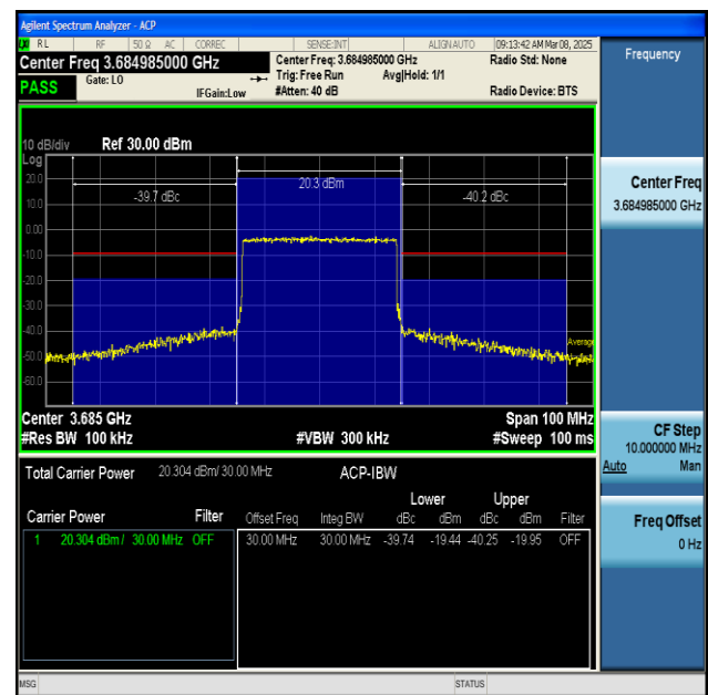
NTNV-n48-PC3-30-30-H-CP-QPSK-Outer_Full-PASS
