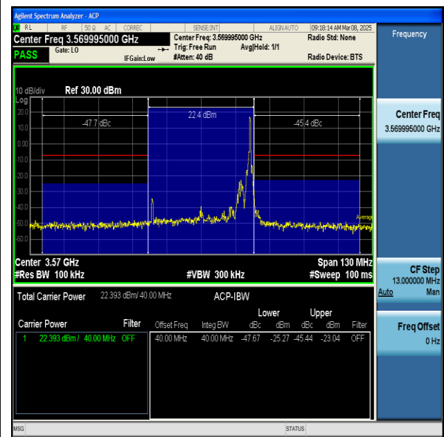
NTVN-n48-PC3-30-40-L-CP-QPSK-Inner_1RB_Right-PASS
