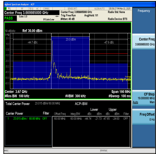
NTNV-n48-PC3-30-60-H-DFT-BPSK-Inner_1RB_Left- PASS
