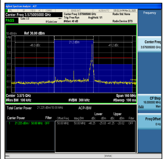
NTVN-n48-PC3-30-50-L-CP-QPSK-Inner_1RB_Right-PASS
