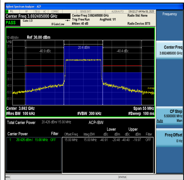
NTNV-n48-PC3-30-15-H-CP-QPSK-Outer_Full-PASS
