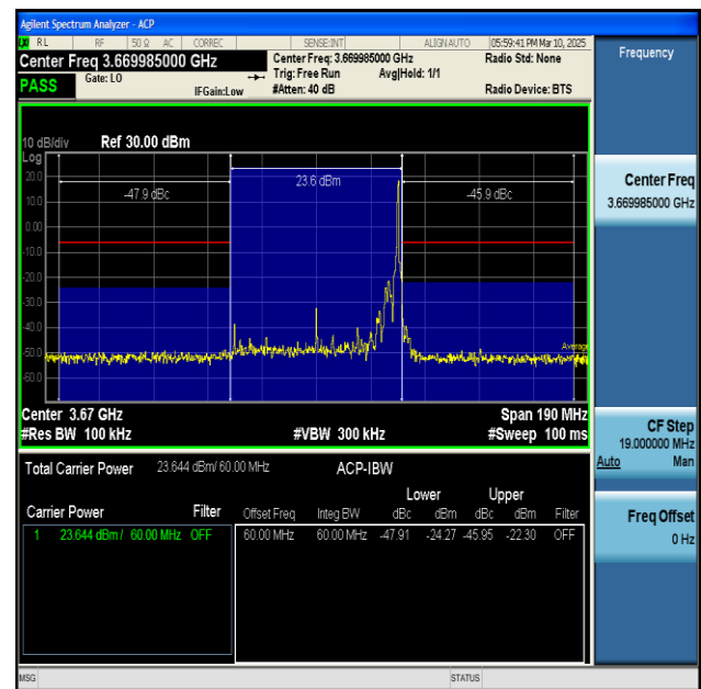
NTNV-n48-PC3-30-60-H-DFT-BPSK-Inner_1RB_Right- PASS
