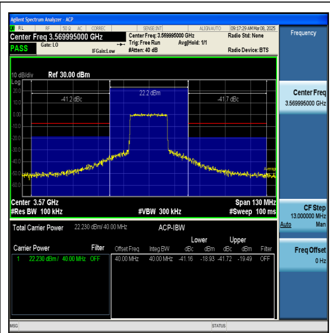
NTNV-n48-PC3-30-40-L-CP-QPSK-Inner_Full-PASS
