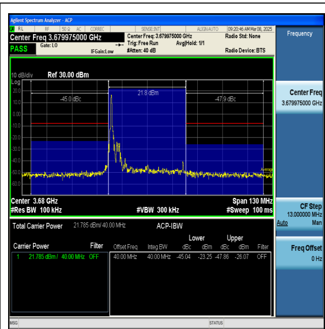
NTNV-n48-PC3-30-40-H-CP-QPSK-Inner_1RB_Left-PASS
