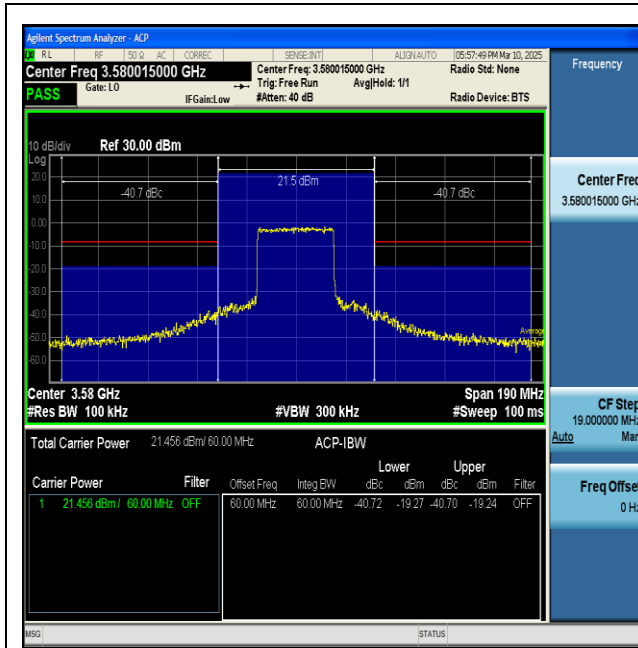
NTNV-n48-PC3-30-60-L-CP-QPSK-Inner_Full-PASS
