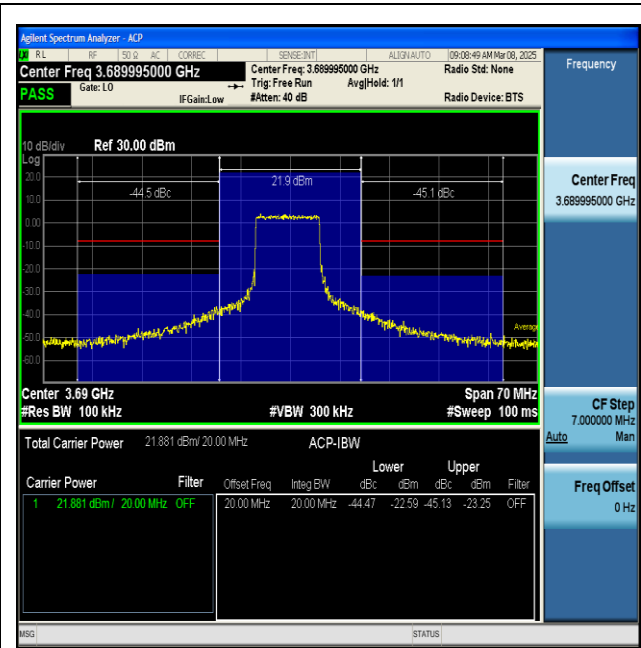
NTNV-n48-PC3-30-20-H-CP-QPSK-Inner_Full-PASS
