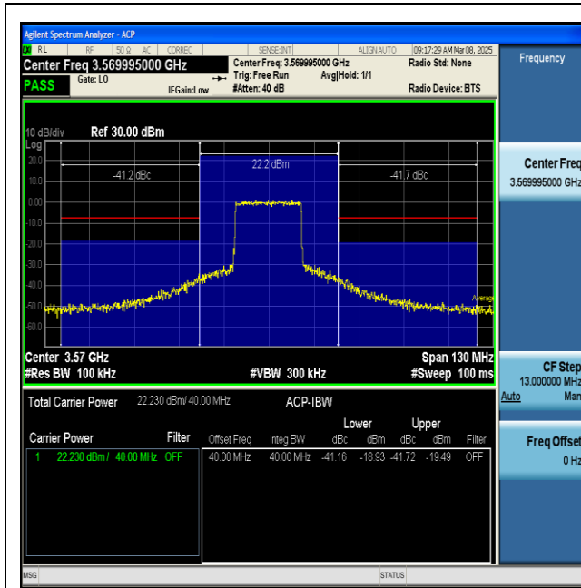
NTNV-n48-PC3-30-40-L-CP-QPSK-Inner_Full-PASS
