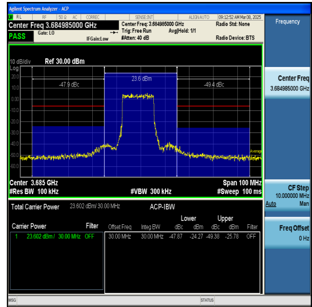
NTNV-n48-PC3-30-30-H-DFT-BPSK-Inner_Full-PASS
