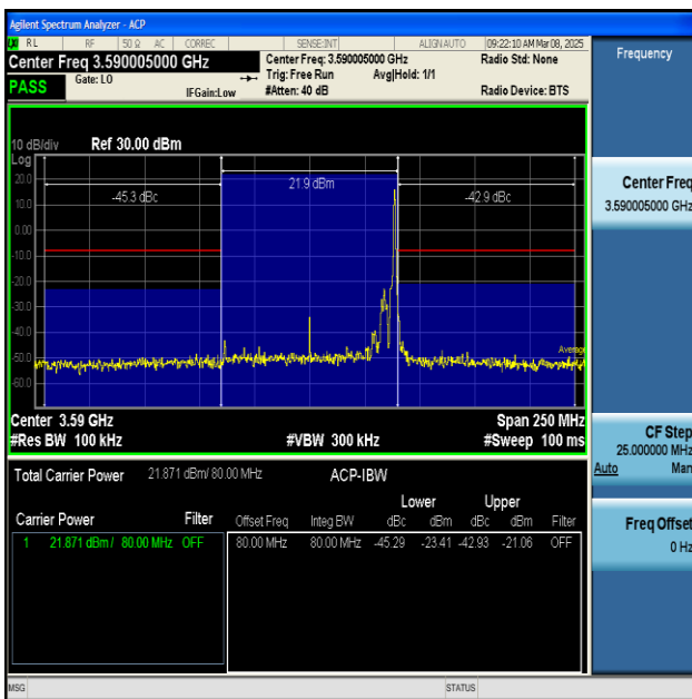
NTNV-n48-PC3-30-80-L-DFT-BPSK-Inner_1RB_Right- PASS
