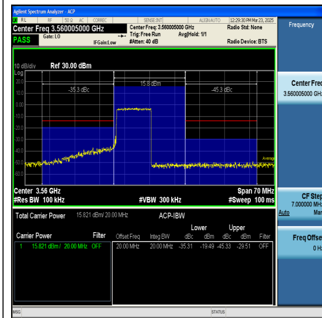
NTNV-n48-PC3-30-20-L-CP-QPSK-Outer_Full-PASS
