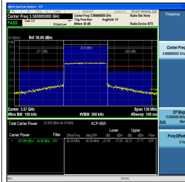
NTNV-n48-PC3-30-40-L-CP-QPSK-Outer_Full-PASS
