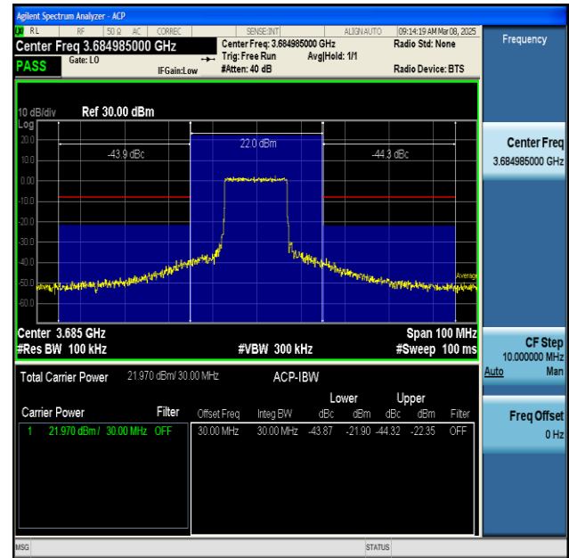
NTNV-n48-PC3-30-30-H-CP-QPSK-Inner_Full-PASS
