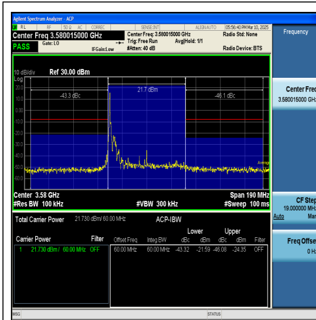
NTNV-n48-PC3-30-60-L-DFT-BPSK-Inner_1RB_Left- PASS
