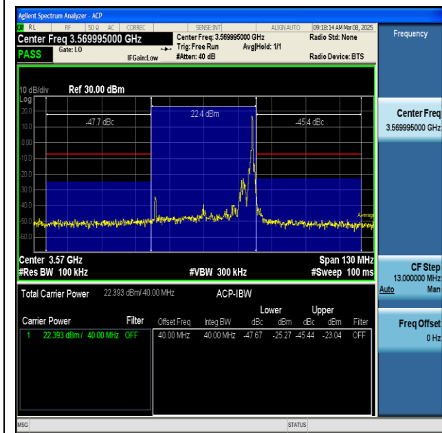
NTVN-n48-PC3-30-40-L-CP-QPSK-Inner_1RB_Right-PASS
