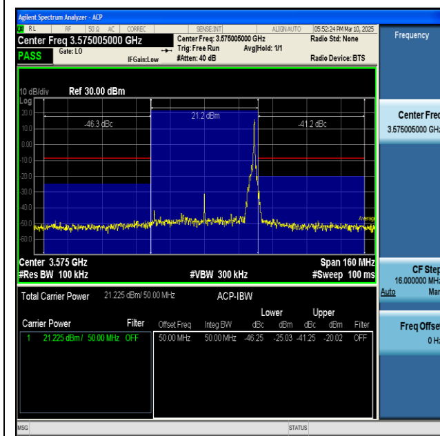
NTVN-n48-PC3-30-50-L-CP-QPSK-Inner_1RB_Right-PASS
