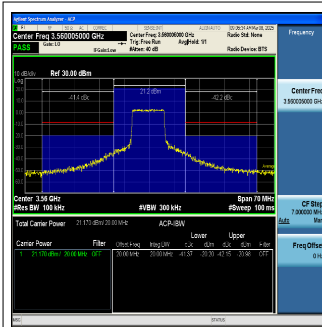
NTNV-n48-PC3-30-20-L-CP-QPSK-Inner_Full-PASS
