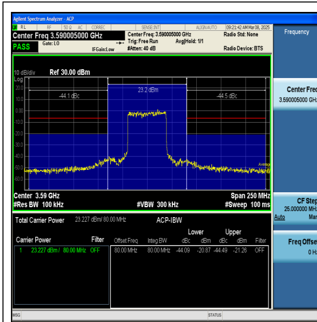
NTNV-n48-PC3-30-80-L-DFT-BPSK-Inner_Full-PASS
