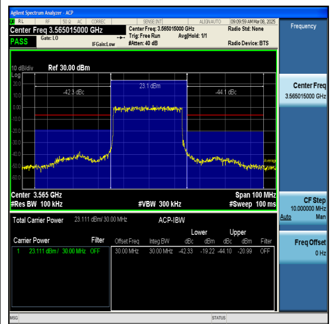
NTNV-n48-PC3-30-30-L-DFT-BPSK-Outer_Full-PASS
