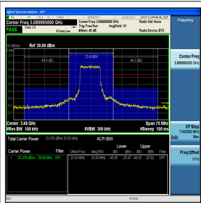
NTNV-n48-PC3-30-20-H-DFT-BPSK-Inner_Full-PASS
