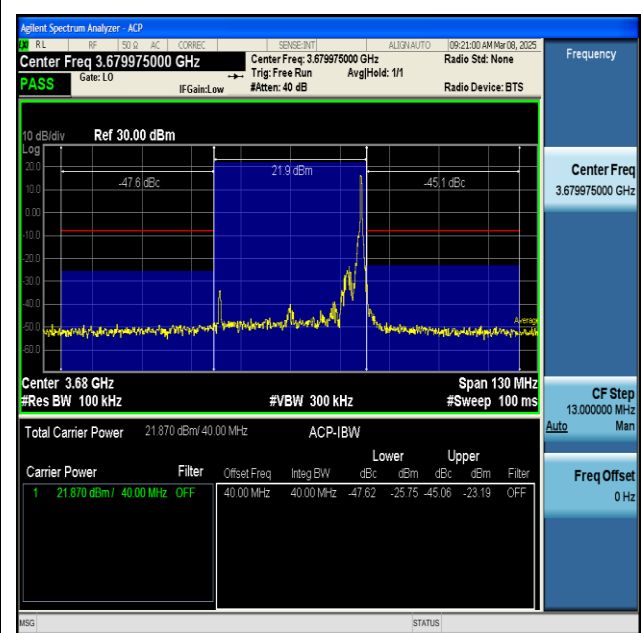
NTNV-n48-PC3-30-40-H-CP-QPSK-Inner_1RB_Right-PASS
