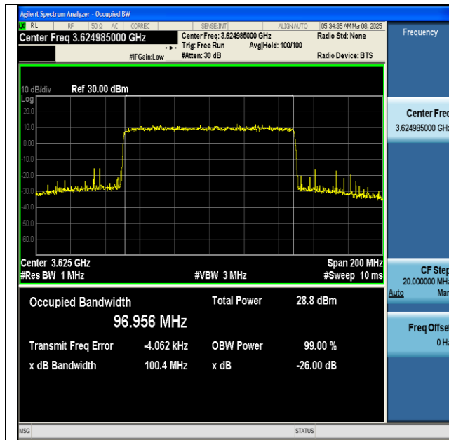
NTNV-n48-PC3-30-100-M-CP-256QAM-Outer_Full-Ant1- PASS
