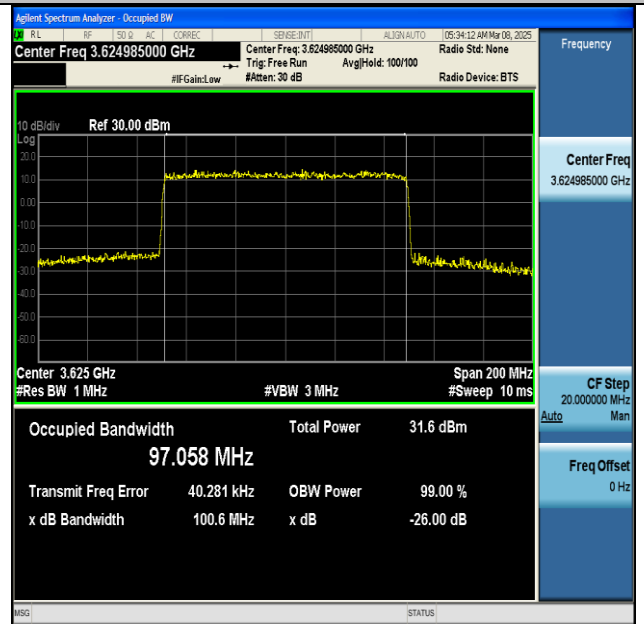
NTVN-n48-PC3-30-100-M-CP-64QAM-Outer_Full-Ant1- PASS
