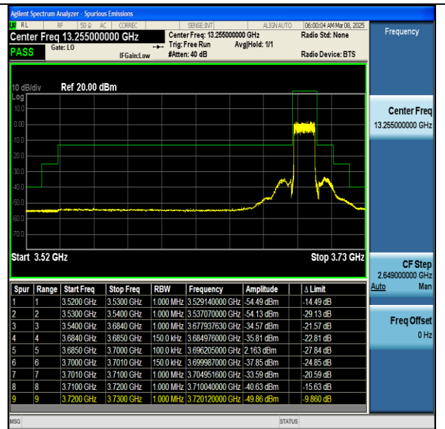
NTNV-n48-PC3-30-15-H-DFT-BPSK-Outer_Full-PASS
