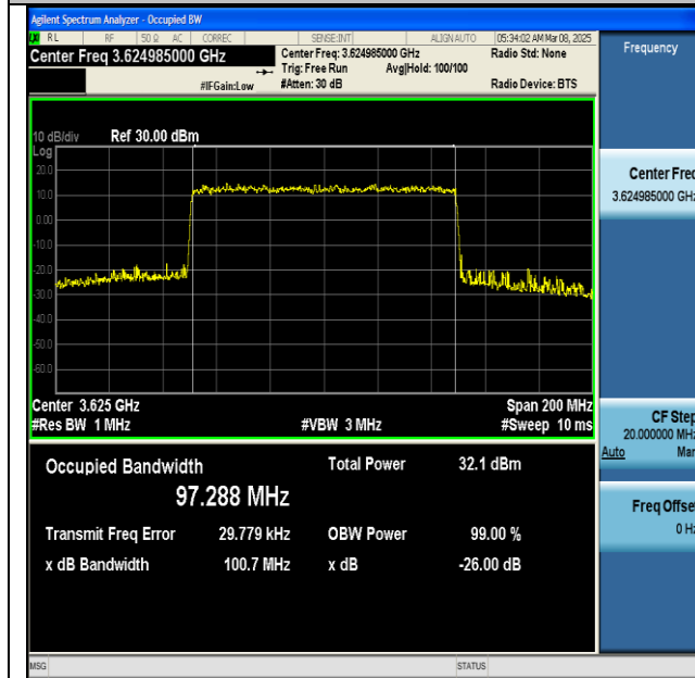
NTVN-n48-PC3-30-100-M-CP-16QAM-Outer_Full-Ant1- PASS
