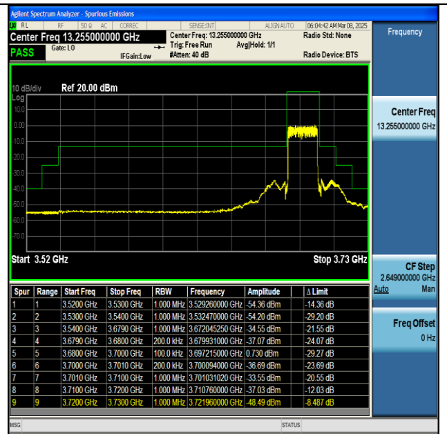
NTNV-n48-PC3-30-20-H-DFT-BPSK-Outer_Full-PASS
