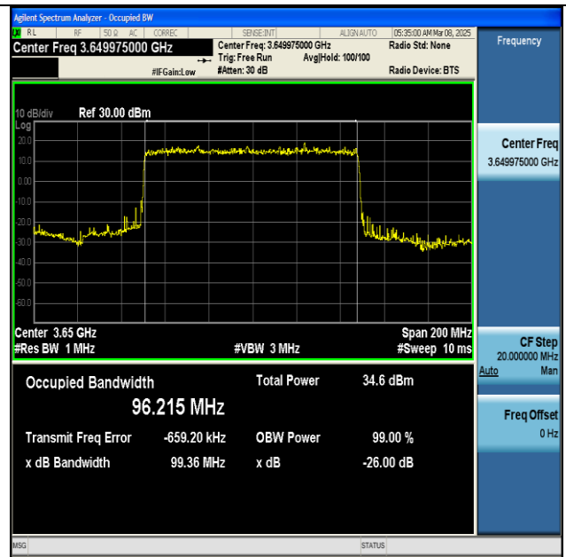
NTNV-n48-PC3-30-100-H-DFT-BPSK-Outer_Full-Ant1- PASS
