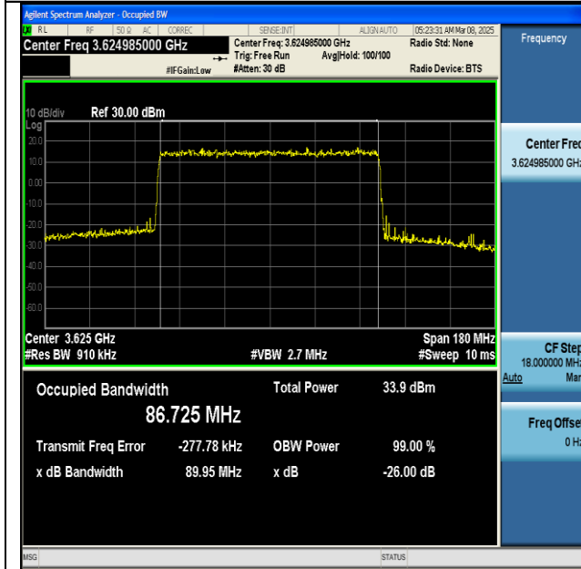
NTNV-n48-PC3-30-90-M-DFT-QPSK-Outer_Full-Ant1- PASS
