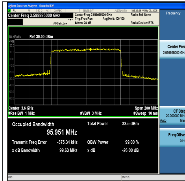
NTNV-n48-PC3-30-100-L-DFT-QPSK-Outer_Full-Ant1- PASS
