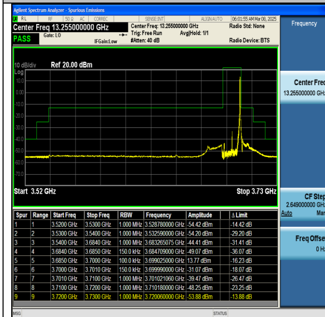
NTNV-n48-PC3-30-15-H-CP-QPSK-Edge_1RB_Right-PASS
