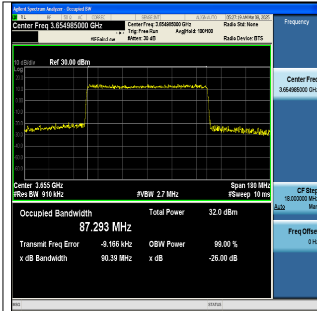
NTNV-n48-PC3-30-90-H-CP-16QAM-Outer_Full-Ant1- PASS
