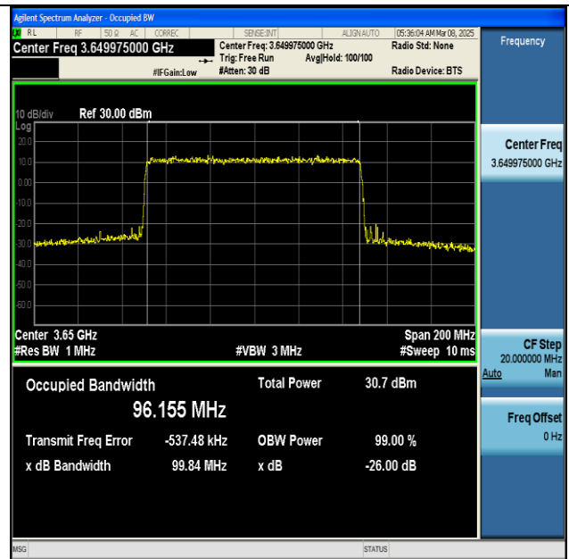
NTNV-n48-PC3-30-100-H-DFT-256QAM-Outer_Full-Ant1- PASS
