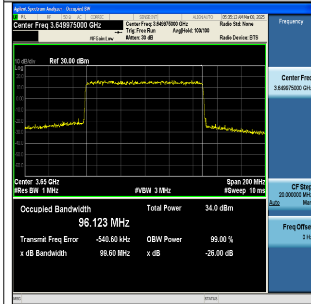
NTNV-n48-PC3-30-100-H-DFT-QPSK-Outer_Full-Ant1- PASS
