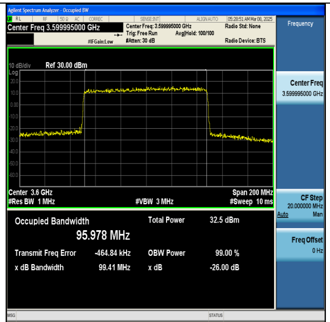
NTNV-n48-PC3-30-100-L-DFT-16QAM-Outer_Full-Ant1- PASS
