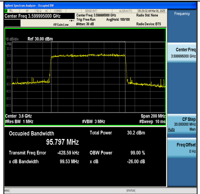
NTNV-n48-PC3-30-100-L-DFT-256QAM-Outer_Full-Ant1- PASS
