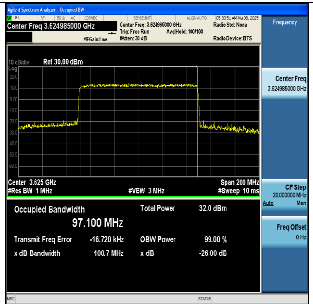
NTVN-n48-PC3-30-100-M-CP-QPSK-Outer_Full-Ant1- PASS
