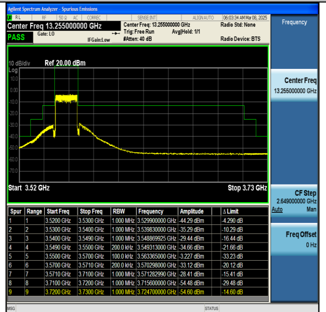
NTNV-n48-PC3-30-20-L-CP-QPSK-Outer_Full-PASS
