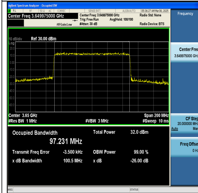
NTNV-n48-PC3-30-100-H-CP-QPSK-Outer_Full-Ant1- PASS
