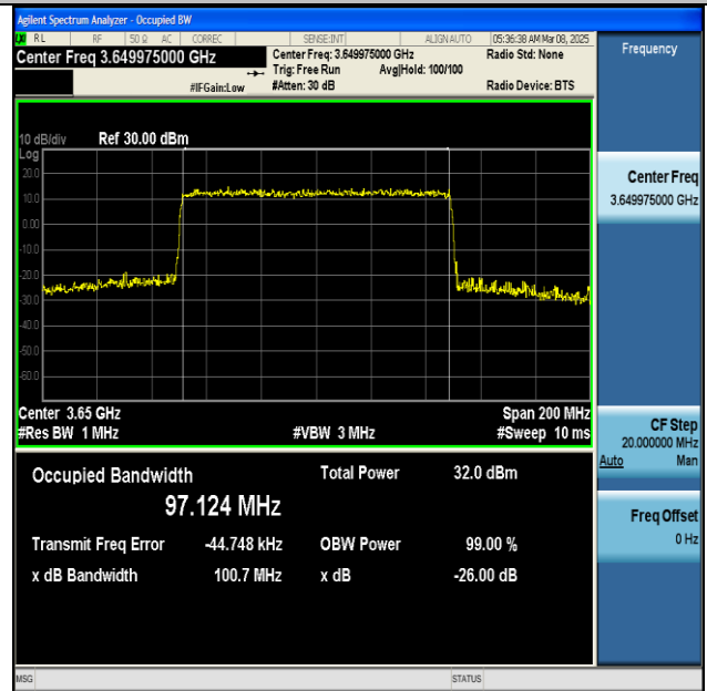
NTNV-n48-PC3-30-100-H-CP-16QAM-Outer_Full-Ant1- PASS
