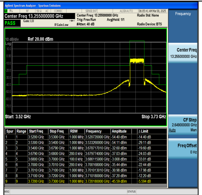
NTNV-n48-PC3-30-20-H-CP-QPSK-Outer_Full-PASS
