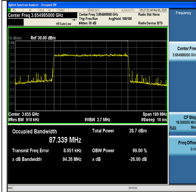
NTNV-n48-PC3-30-90-H-CP-256QAM-Outer_Full-Ant1- PASS
