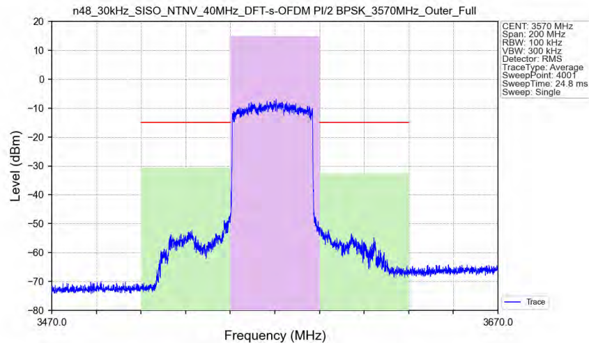
n48_30kHz_SISO_NTNV_40MHz_DFT-s-OFDM PI/2 BPSK_3570MHz_Outer_Full_Ant1
