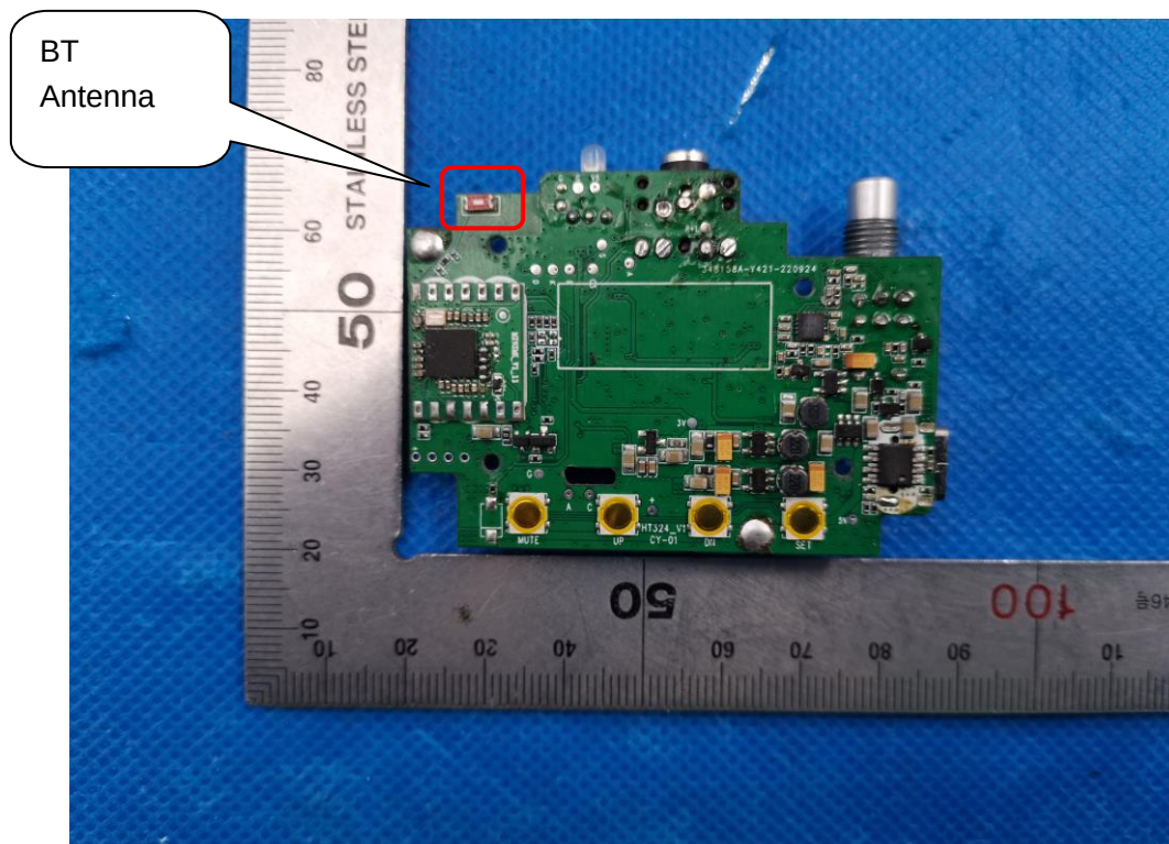
INTERNAL VIEW OF EUT (FIGURE 2)
