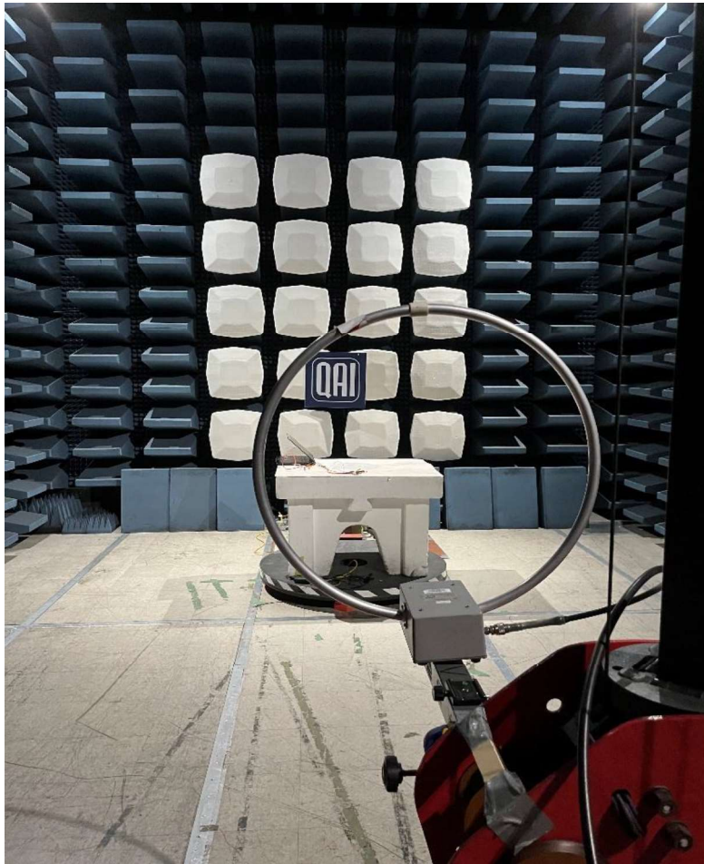
Figure 32: Radiated Emissions performed at the 3m SAC, 150kHz – 30MHz
