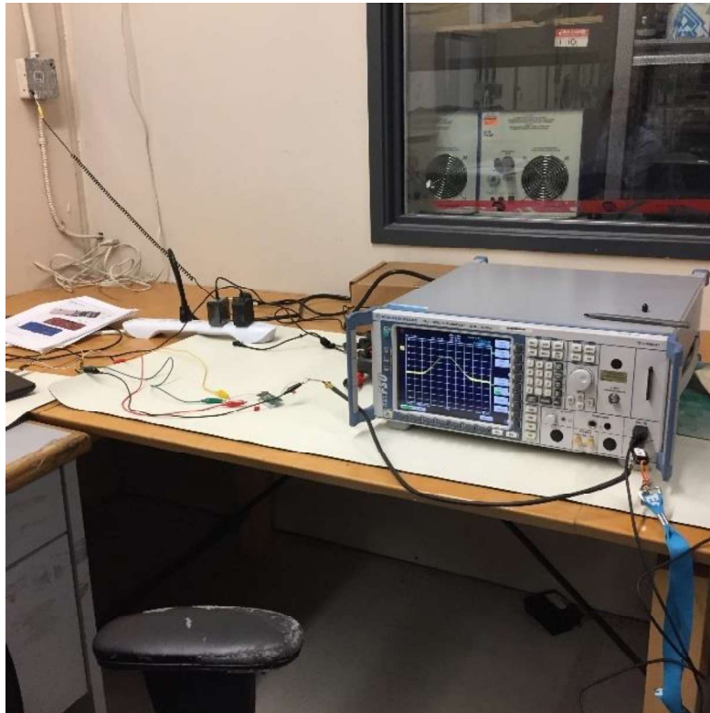
Figure 29: Radio Testing Setup Photo
